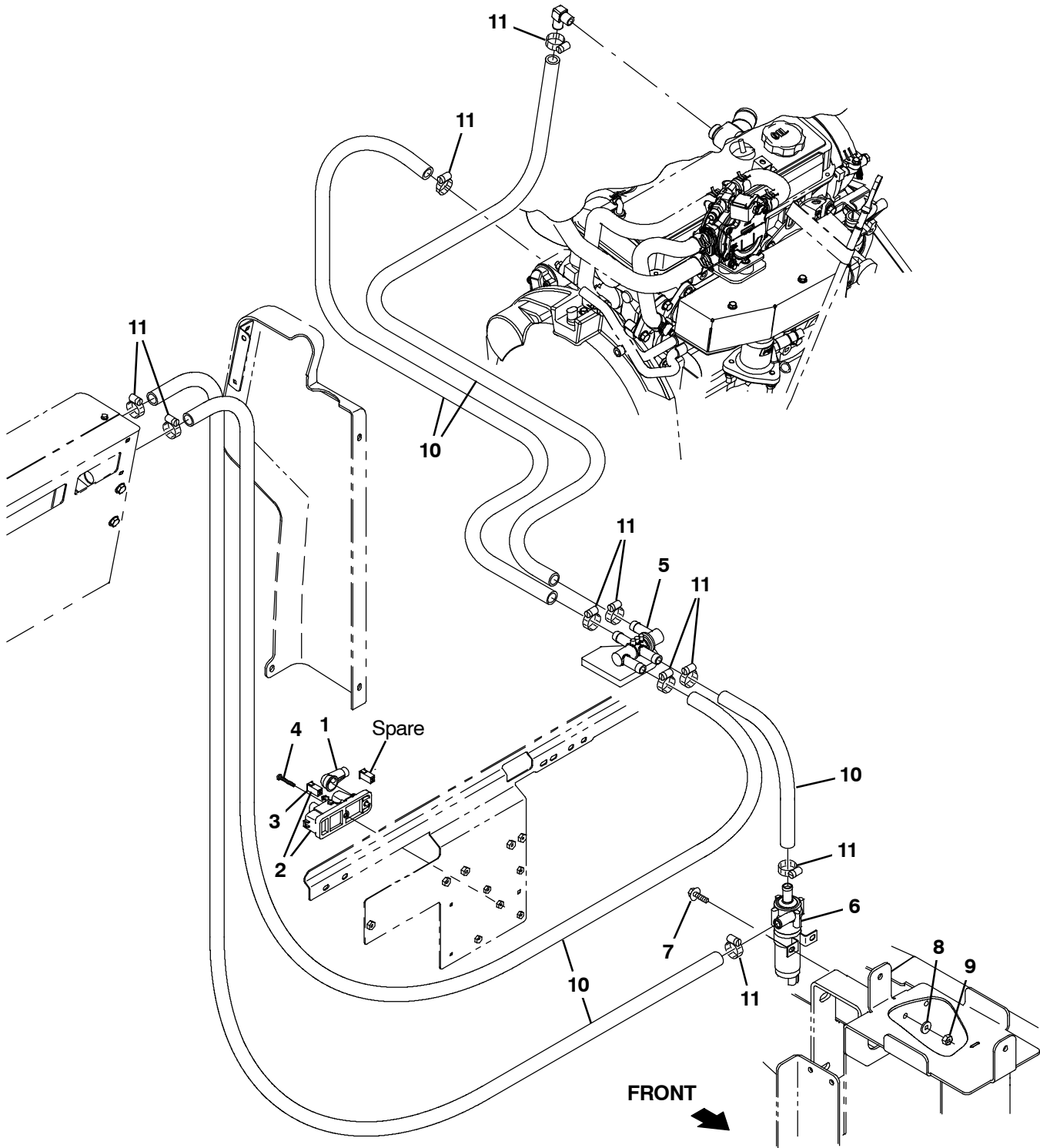
Fig. 9 - Cab Heater Group
