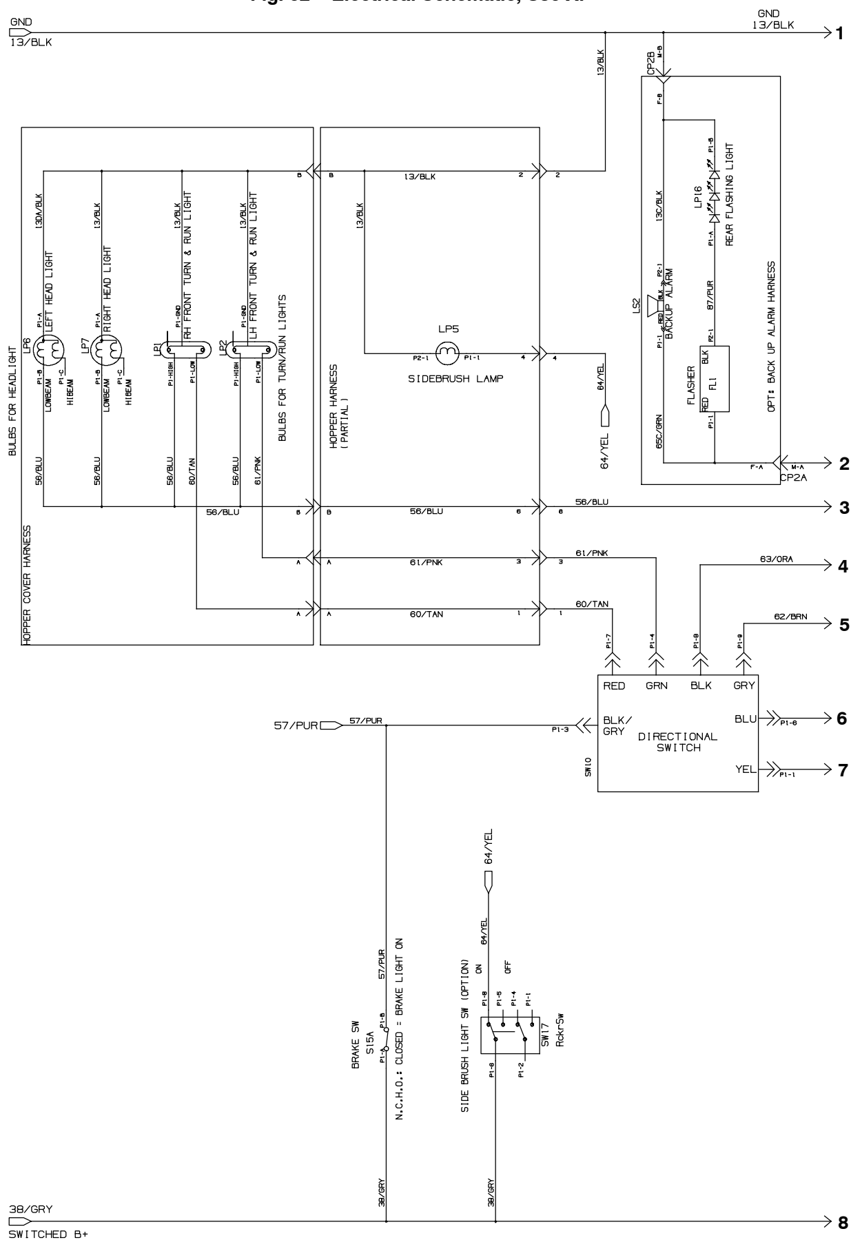
Fig. 62 - Electrical Schematic, S30 XP
