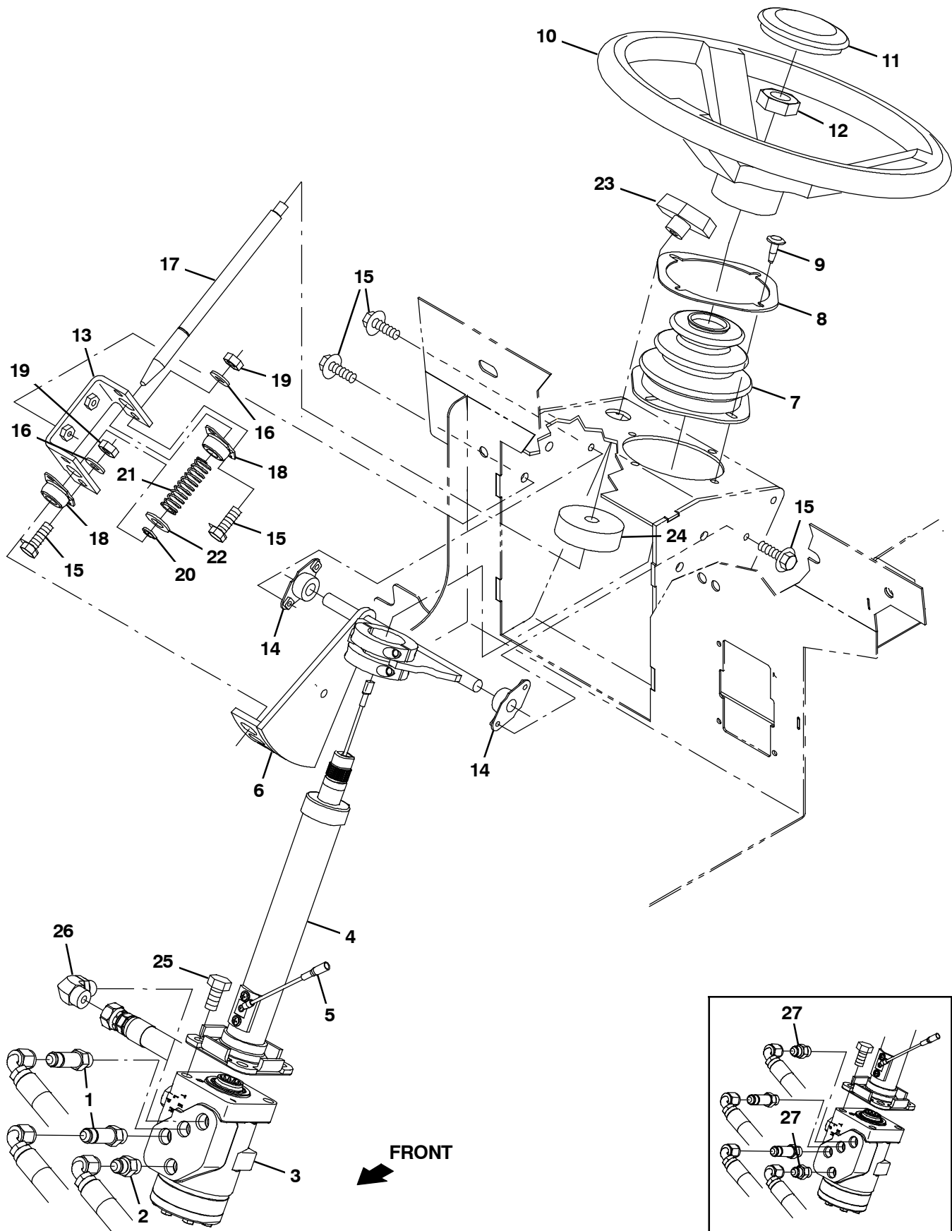
Fig. 12 - Steering Group
