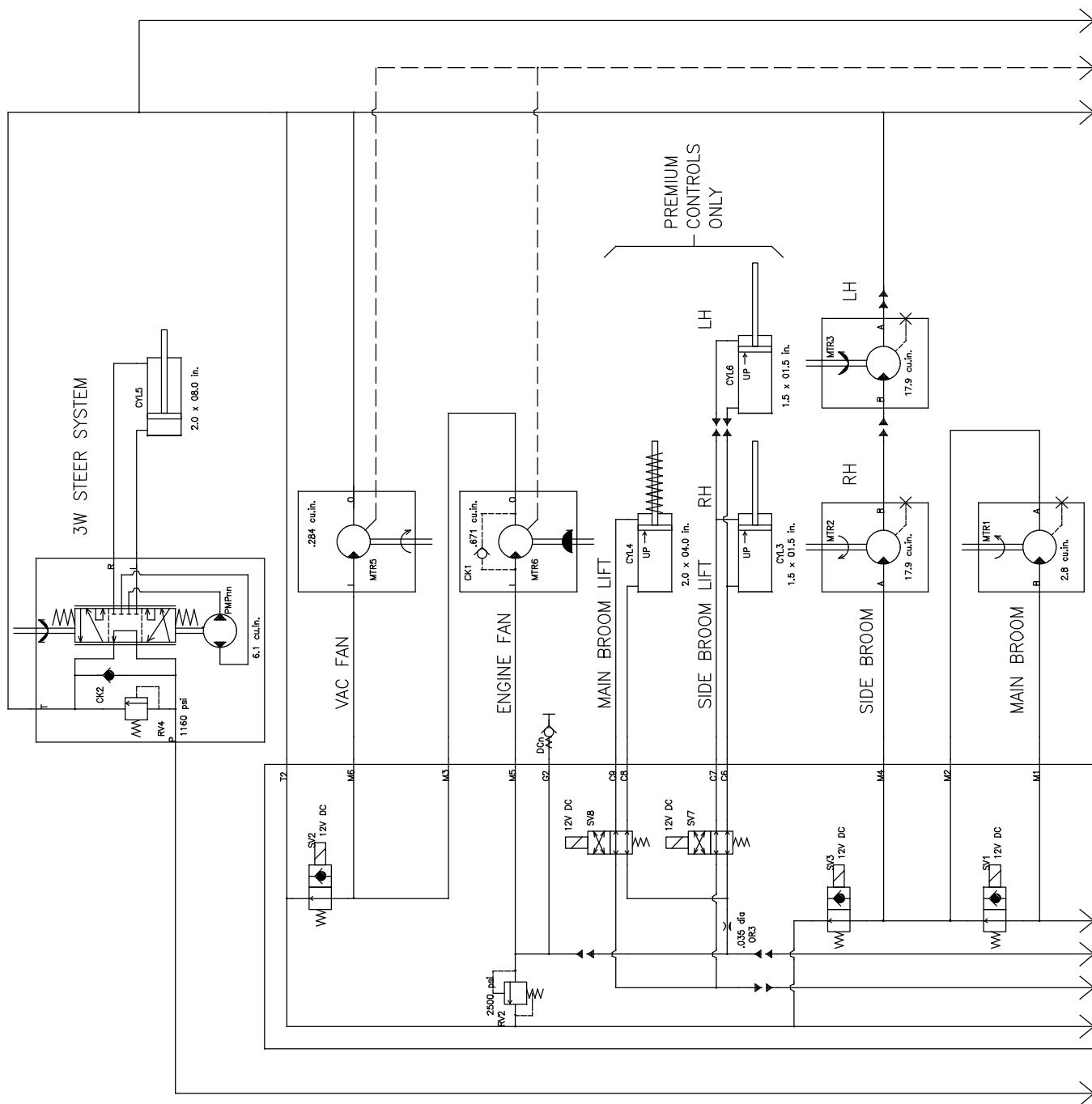
Fig. 52 - Hydraulic Schematic (S/N 011079- )
