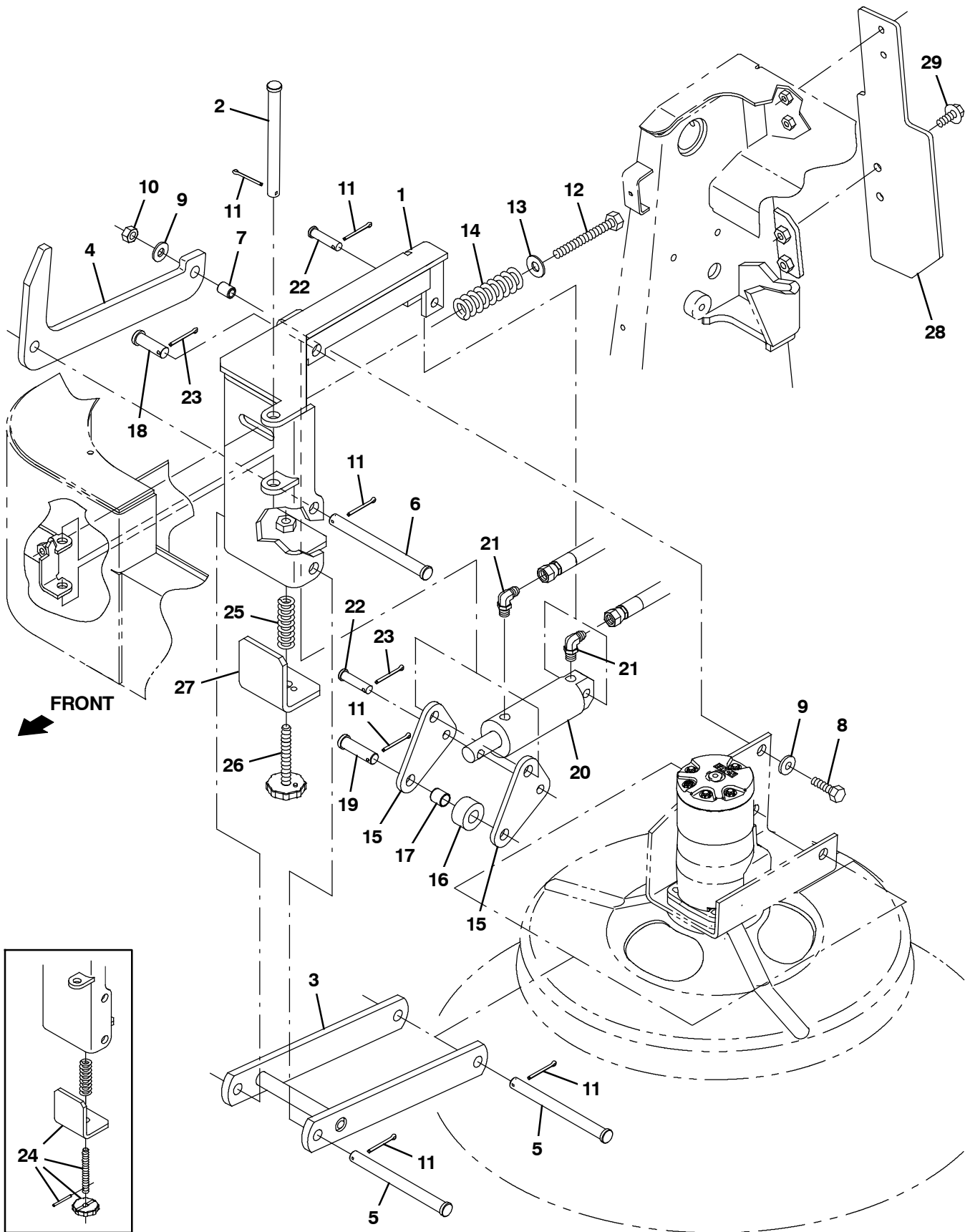
Fig. 47 - Side Brush Lift and Pivot Group, S30 XP
