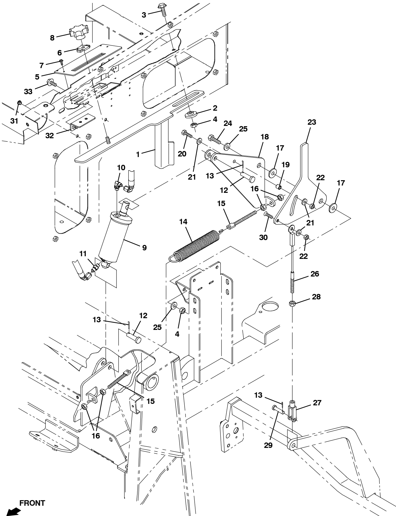
Fig. 49 - Main Brush Lift Group, S30 XP
