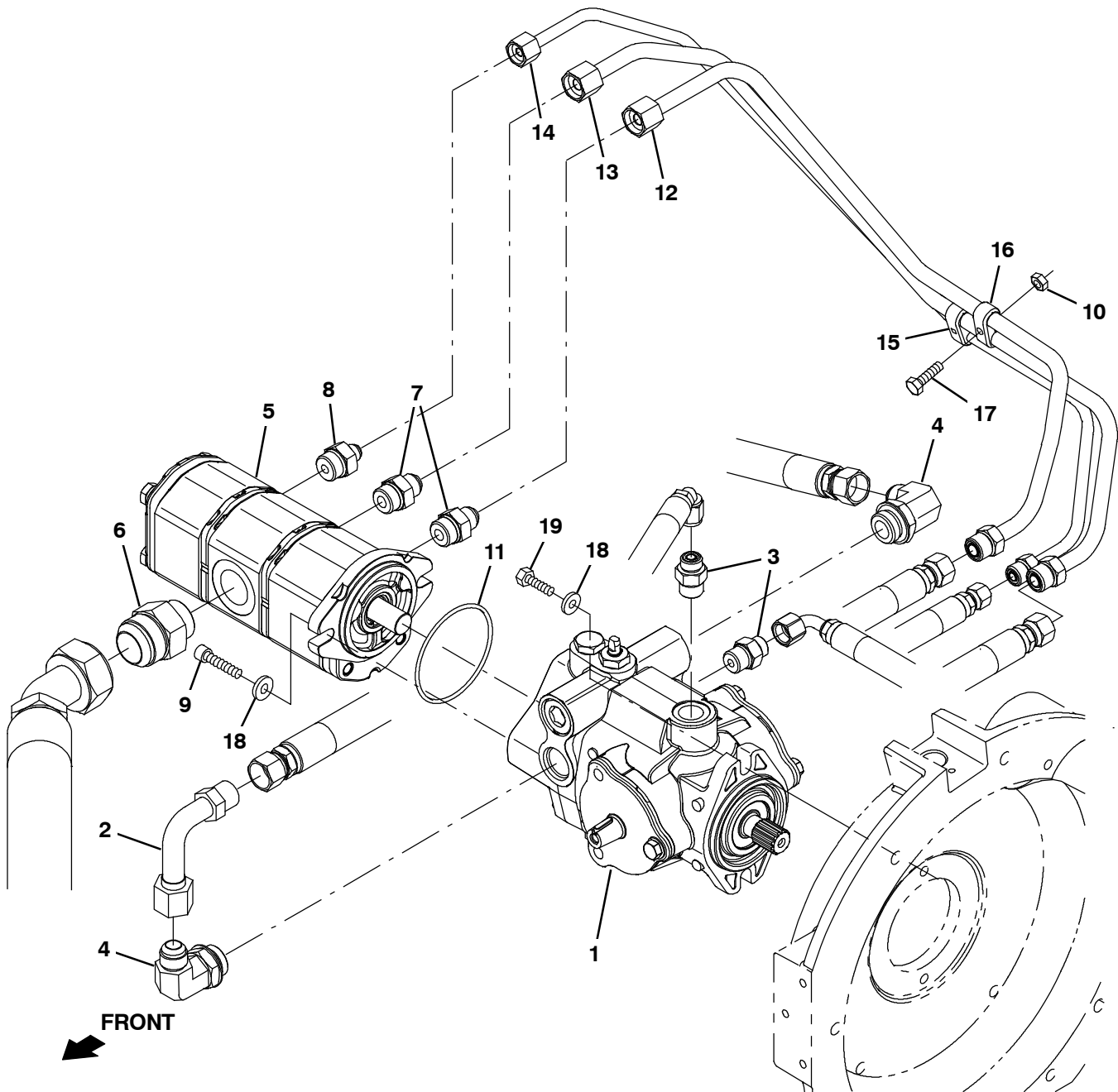
Fig. 58 - Hydraulic Pumps Group, S30 and XP (S/N 011079- )
