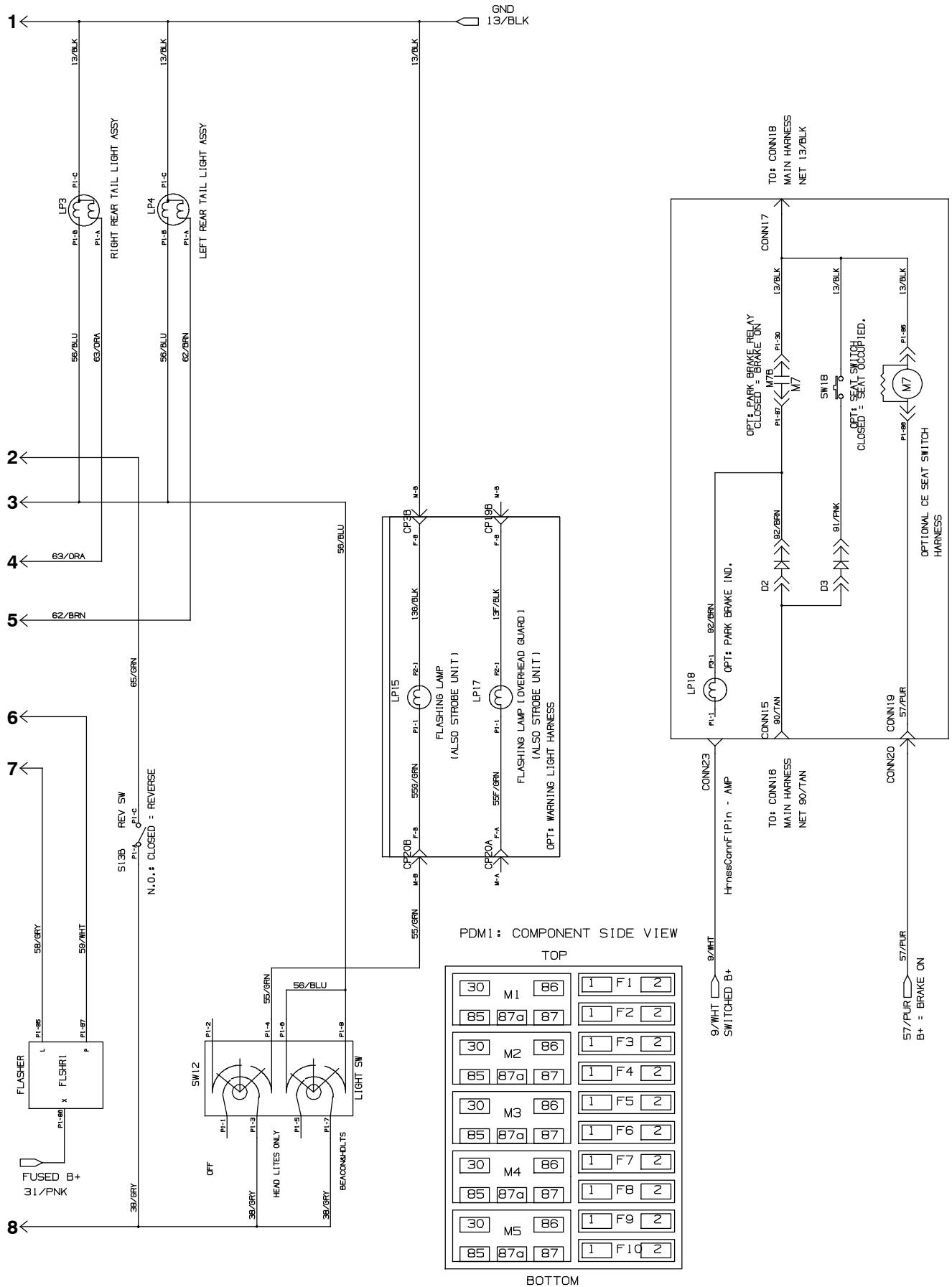
Fig. 62 - Electrical Schematic, S30 XP
