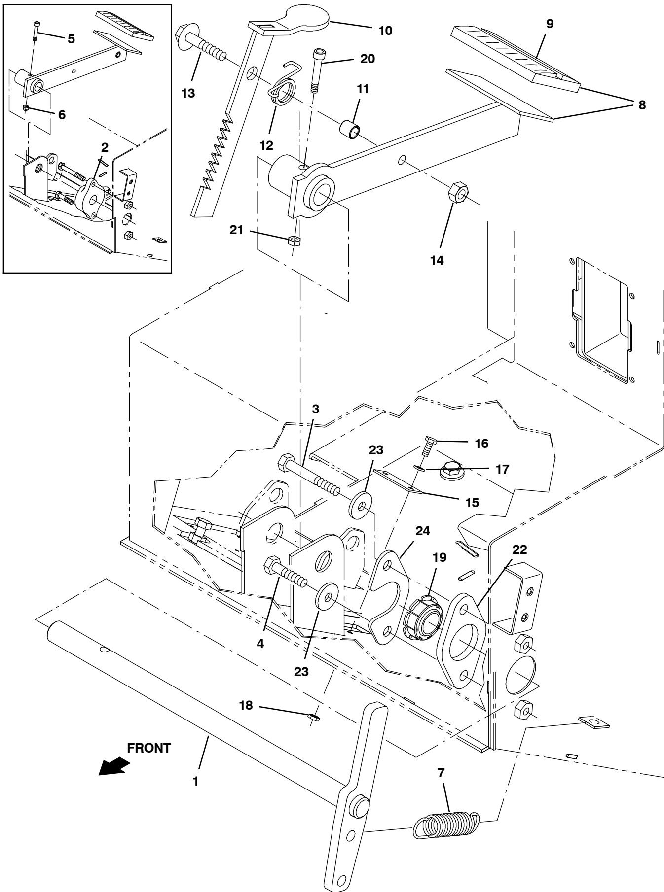
Fig. 30 - Brake Pedal and Parking Brake Group
