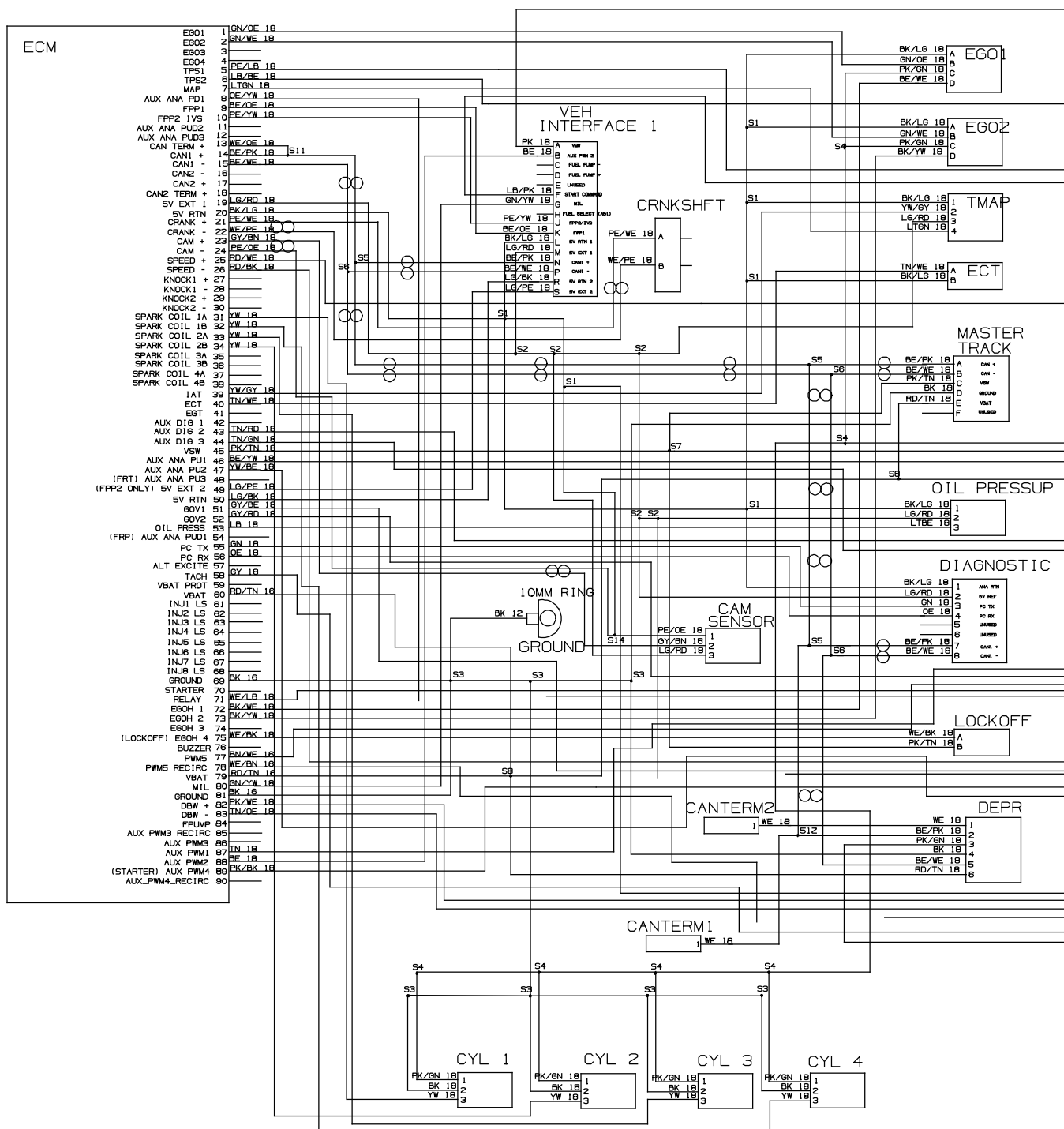
Fig. 64 - Electrical Schematic, LPG Engine Harness (1 of 2)
