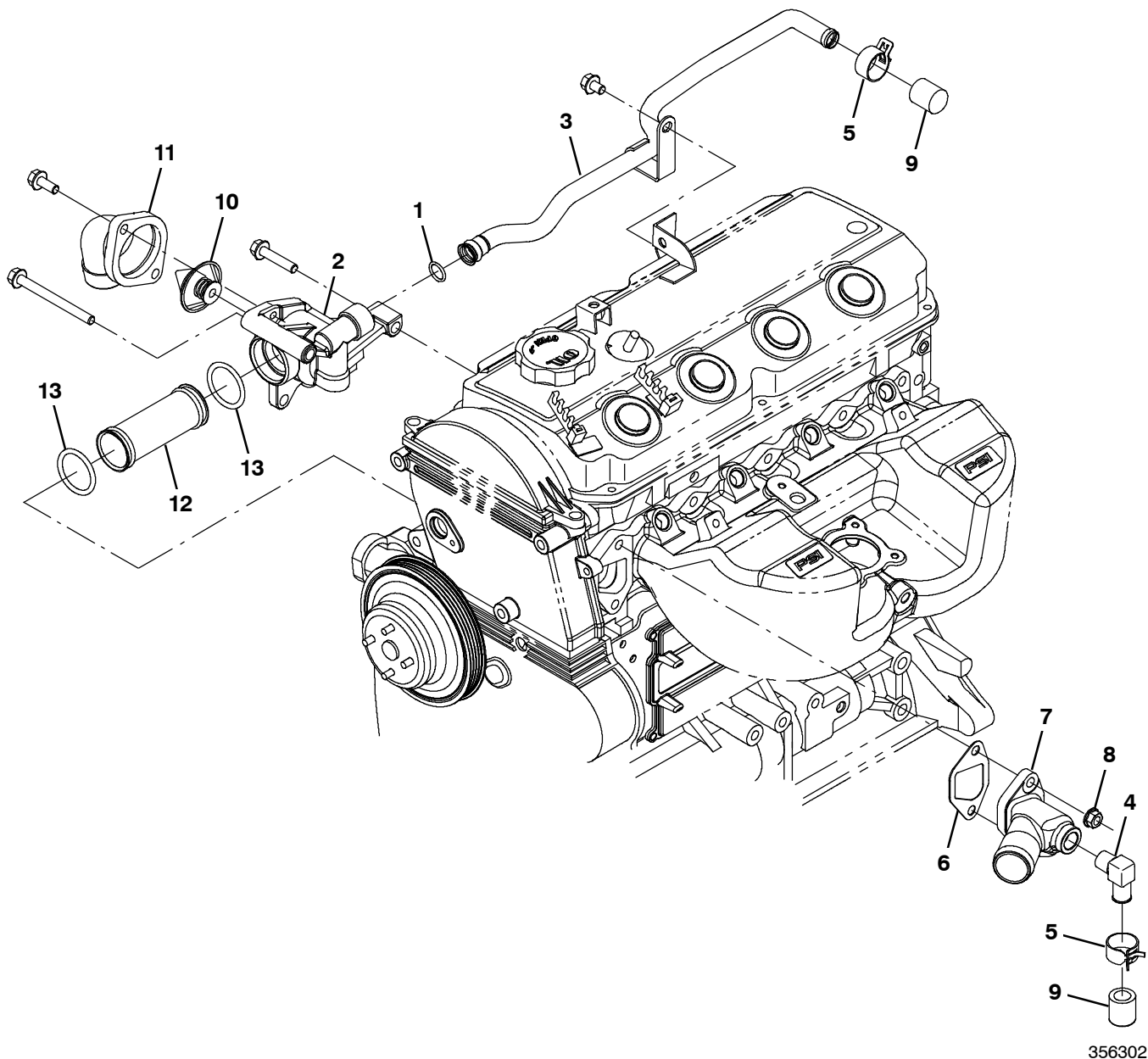
Fig. 17 - Coolant Group
