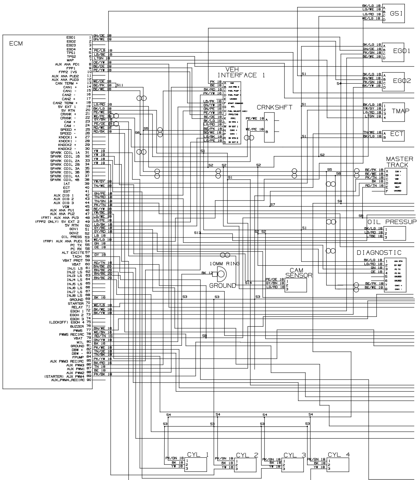
Fig. 63 - Electrical Schematic, Gas Engine Harness (1 of 2)
