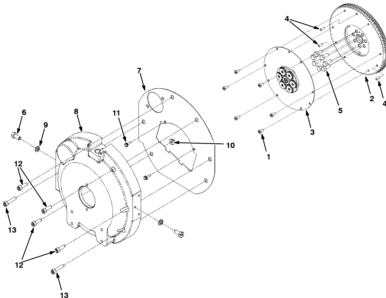
Fig. 13 - Flywheel Group
