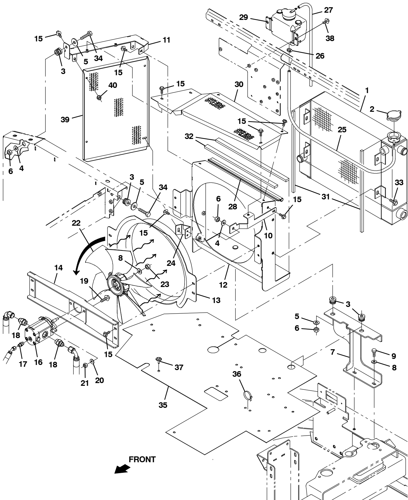
Fig. 24 - Engine Radiator Mount and Fan Group
