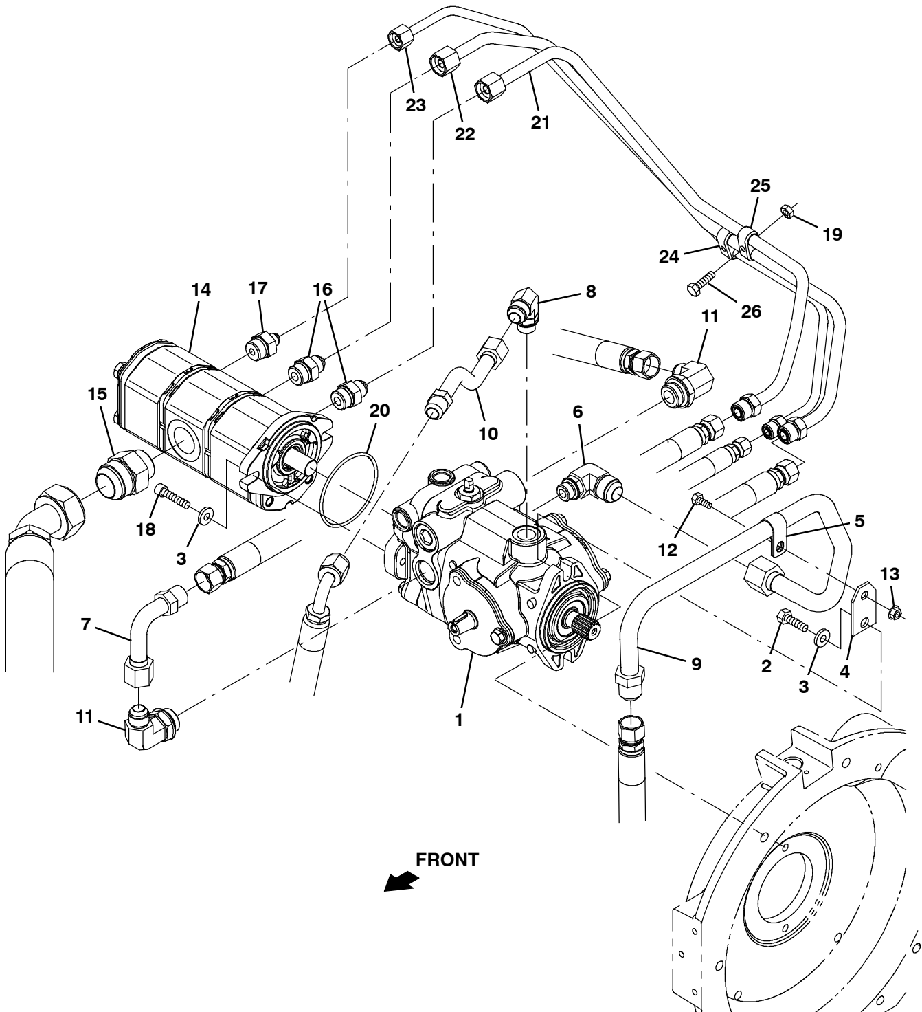
Fig. 57 - Hydraulic Pumps Group, S30 and XP (S/N 006501 - 011078)
