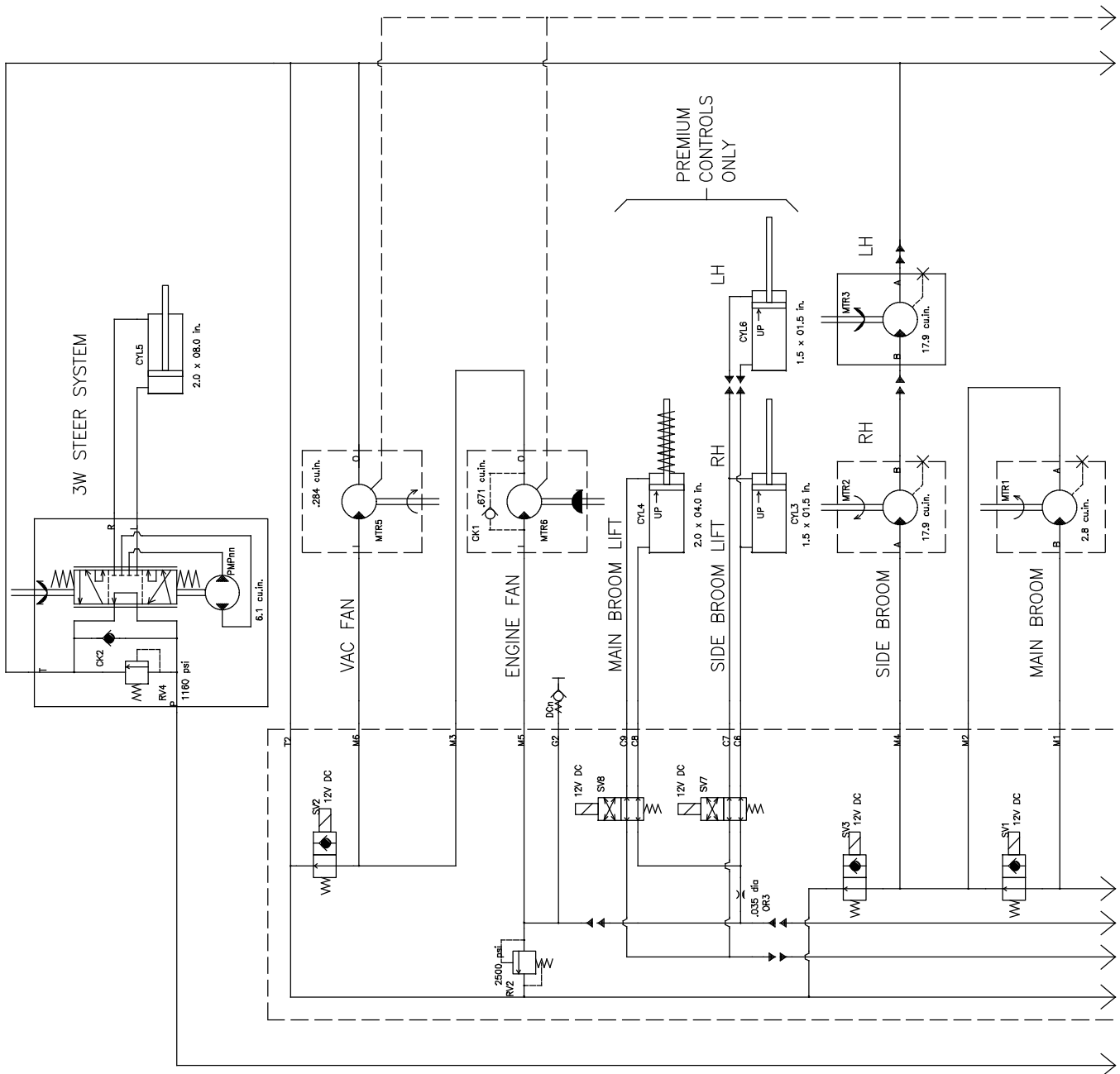
Fig. 51 - Hydraulic Schematic (S/N 006501-011078)
