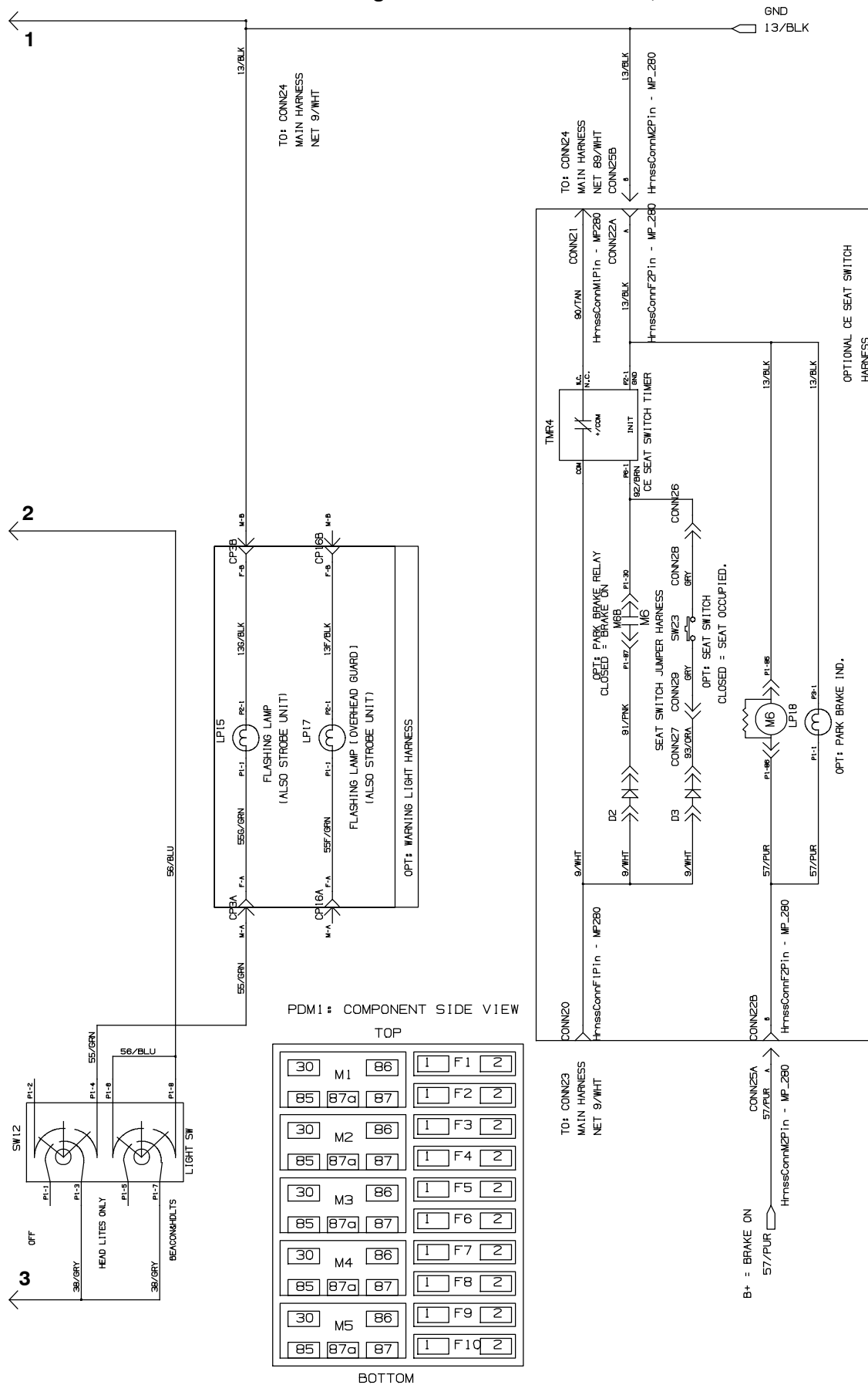
Fig. 61 - Electrical Schematic, S30
