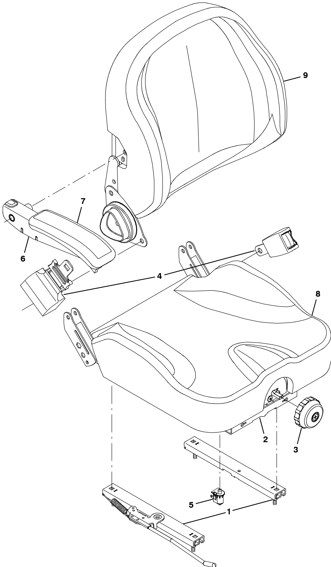
Fig. 7 - Seat Breakdown, 9018735
