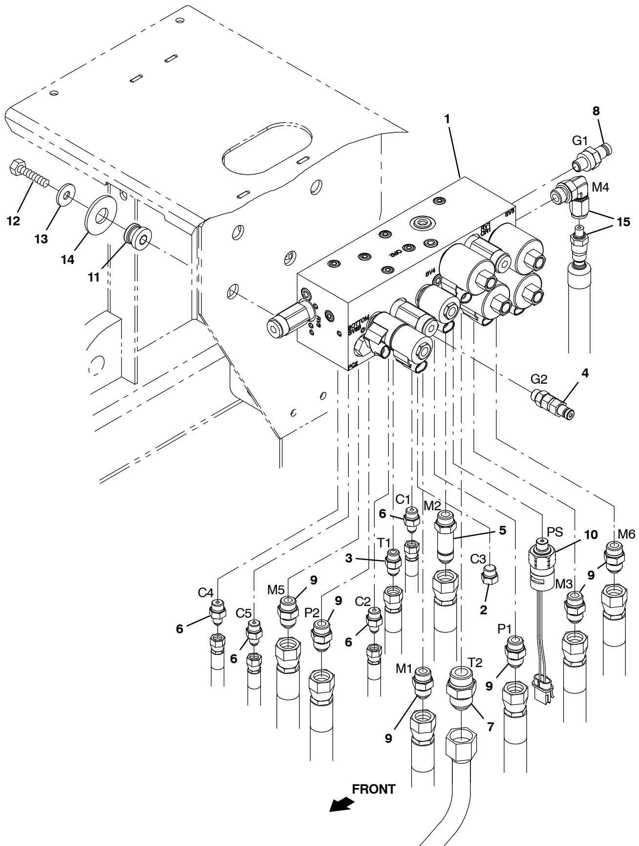
Fig. 59 - Hydraulic Valve Group, S30
