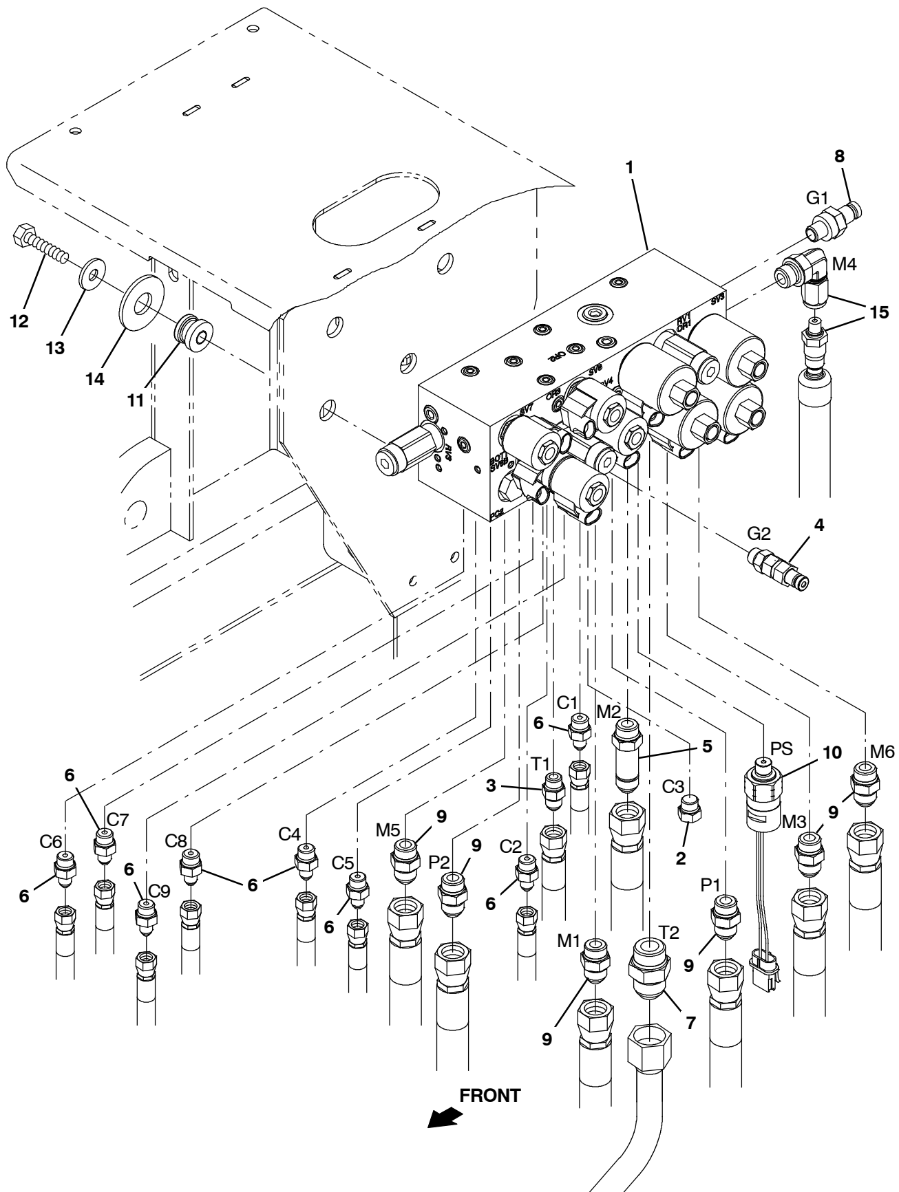
Fig. 60 - Hydraulic Valve Group, S30 XP
