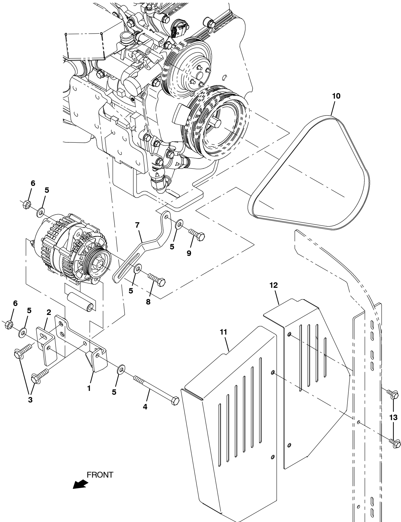
Fig. 19 - Engine Alternator Group
