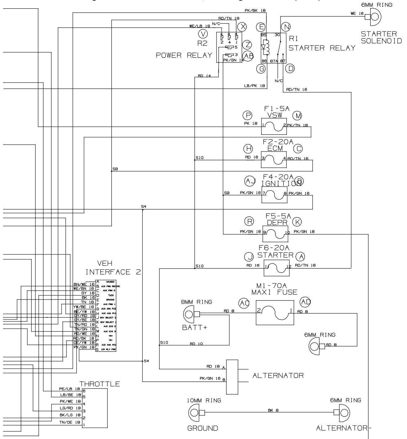
Fig. 64 - Electrical Schematic, LPG Engine Harness (2 of 2)
