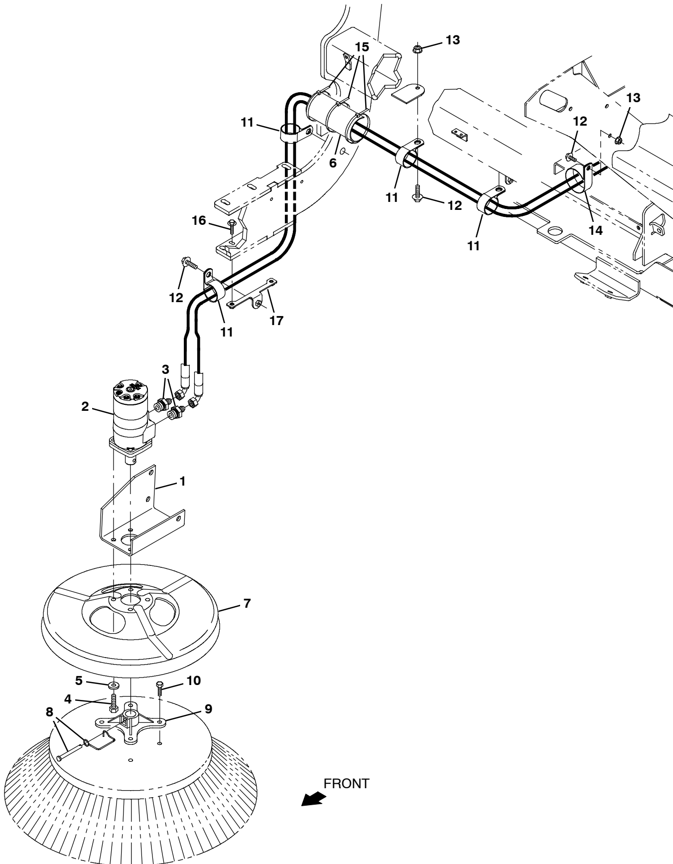
Fig. 46 - Side Brush Motor Group, S30 XP
