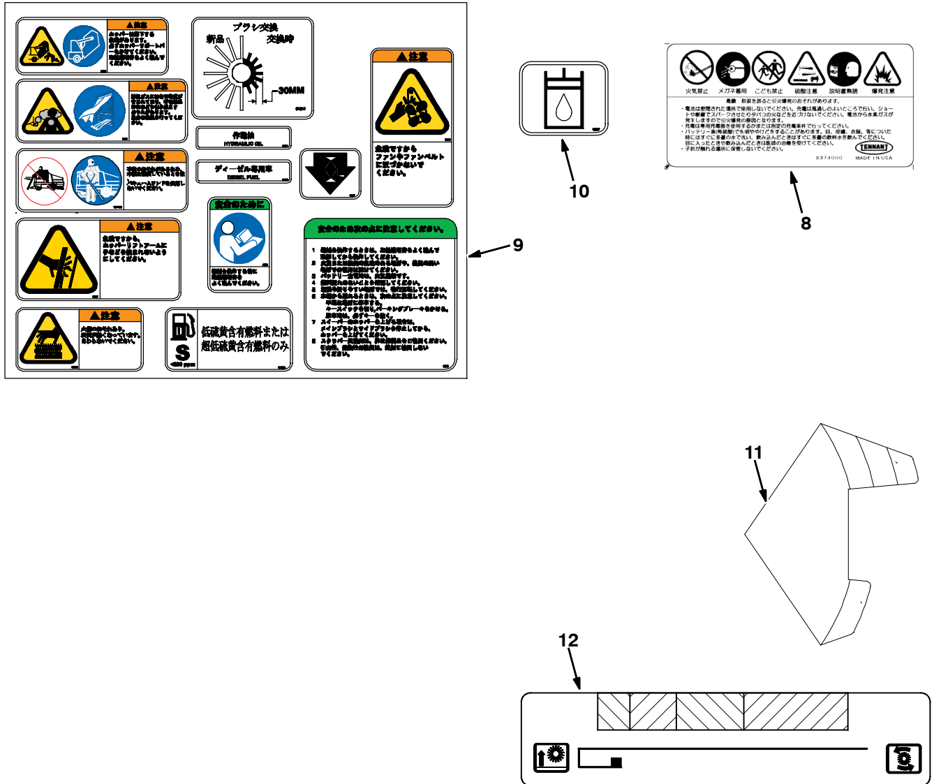
Fig. 66 - Label Group
