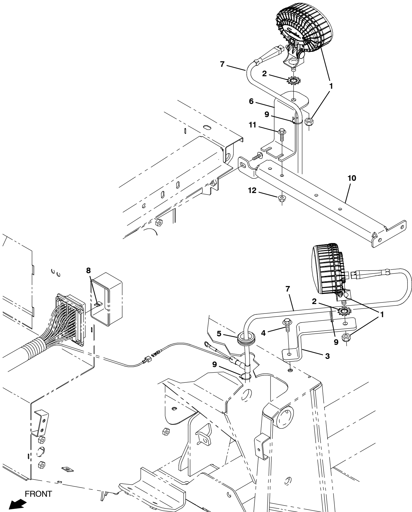
Fig. 32 - Spotlight Kit, Blue
