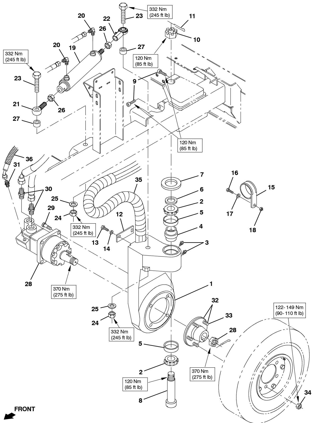
Fig. 26 - Wheel Group, Rear Drive S30 and XP
