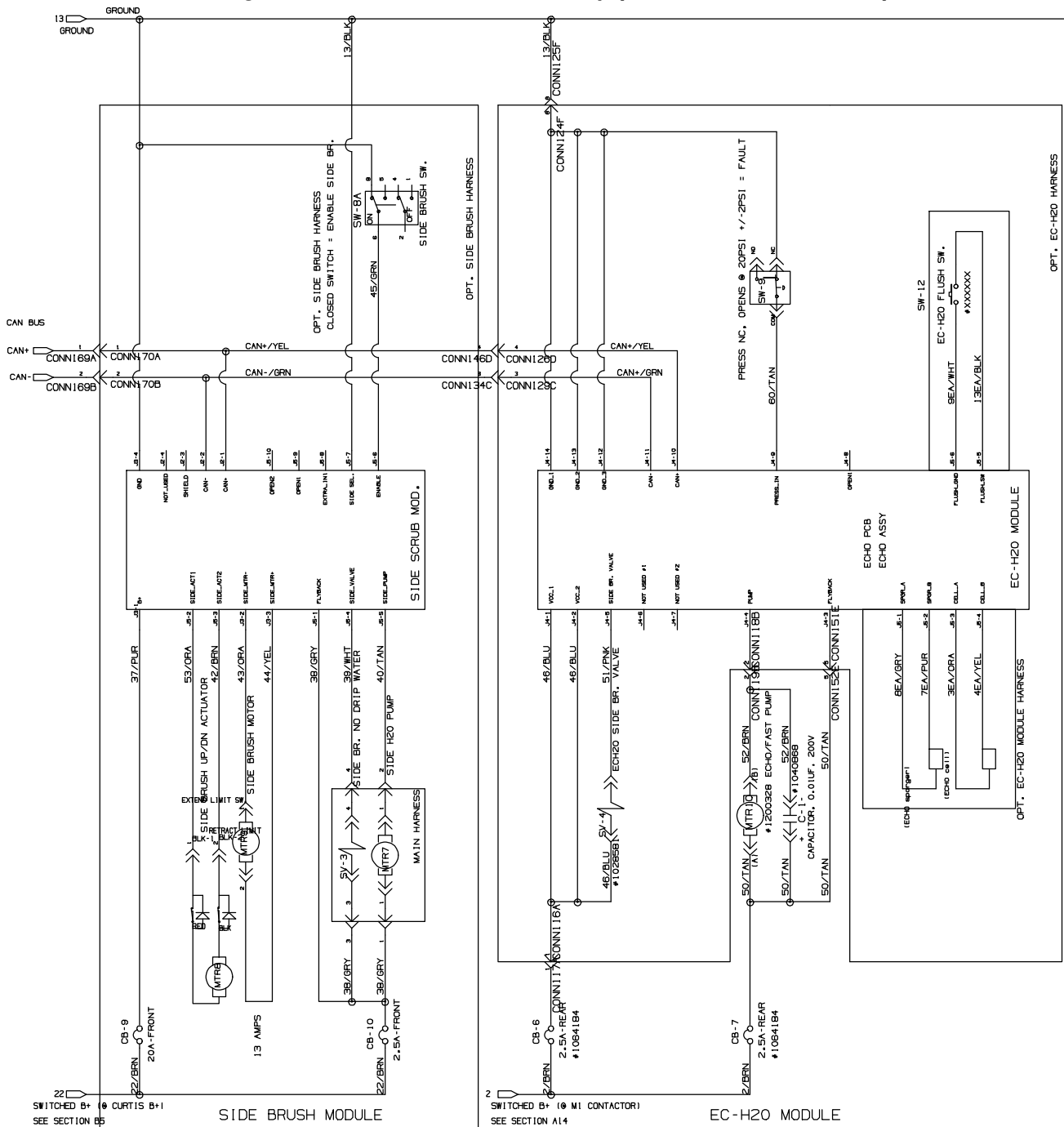
Fig. 25 – Electrical Schematic Group (S/N 30000000–30077834)
