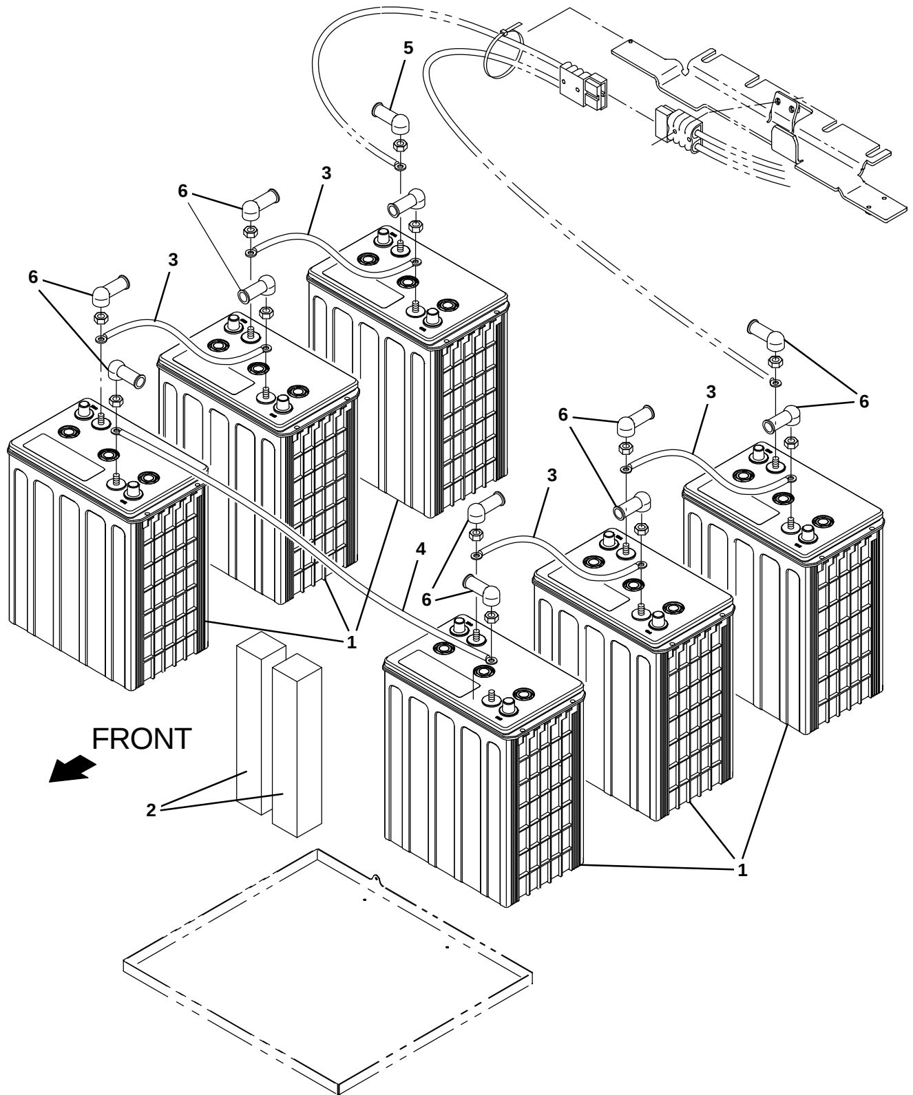
Fig. 20 – Battery Group, 36V 312Ah
