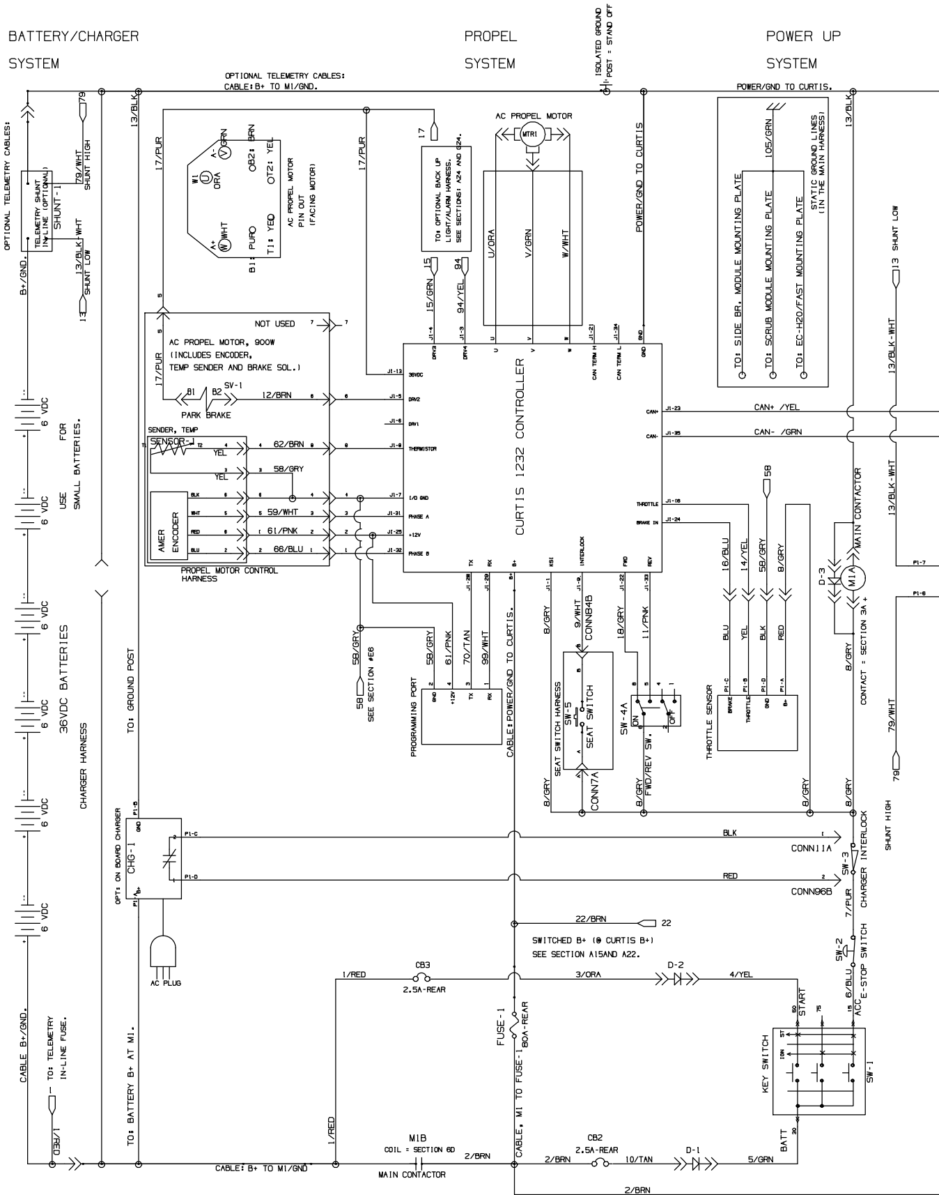
Fig. 25 – Electrical Schematic Group (S/N 30000000–30077834)
