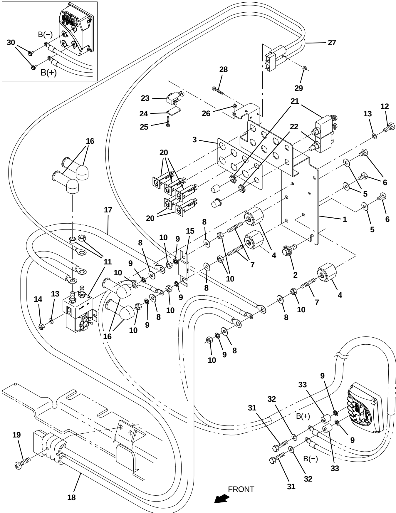
Fig. 23 – Electrical Contactor and Wires Group
