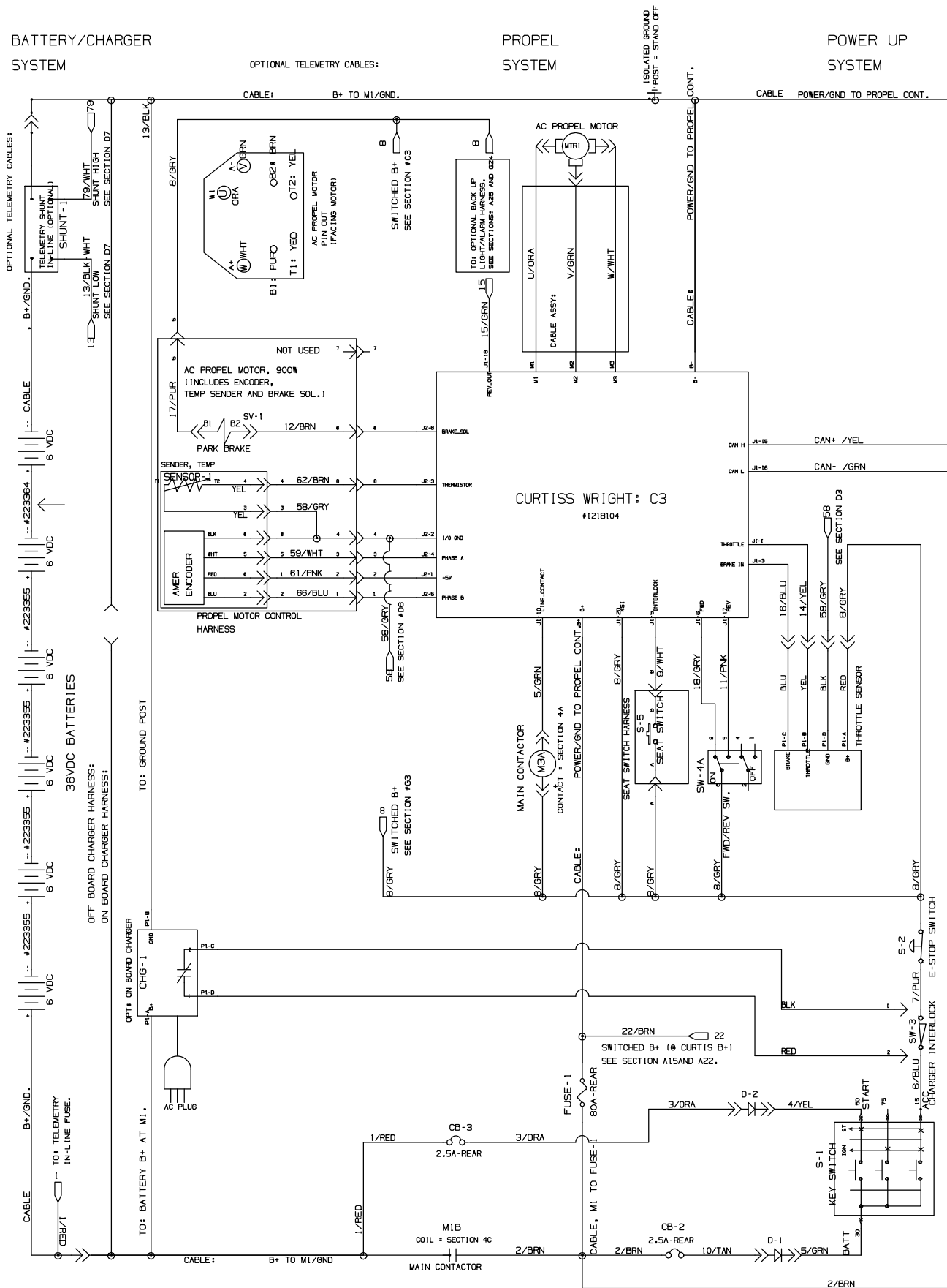
Fig. 26 – Electrical Schematic Group (S/N 30077835–39999999)
