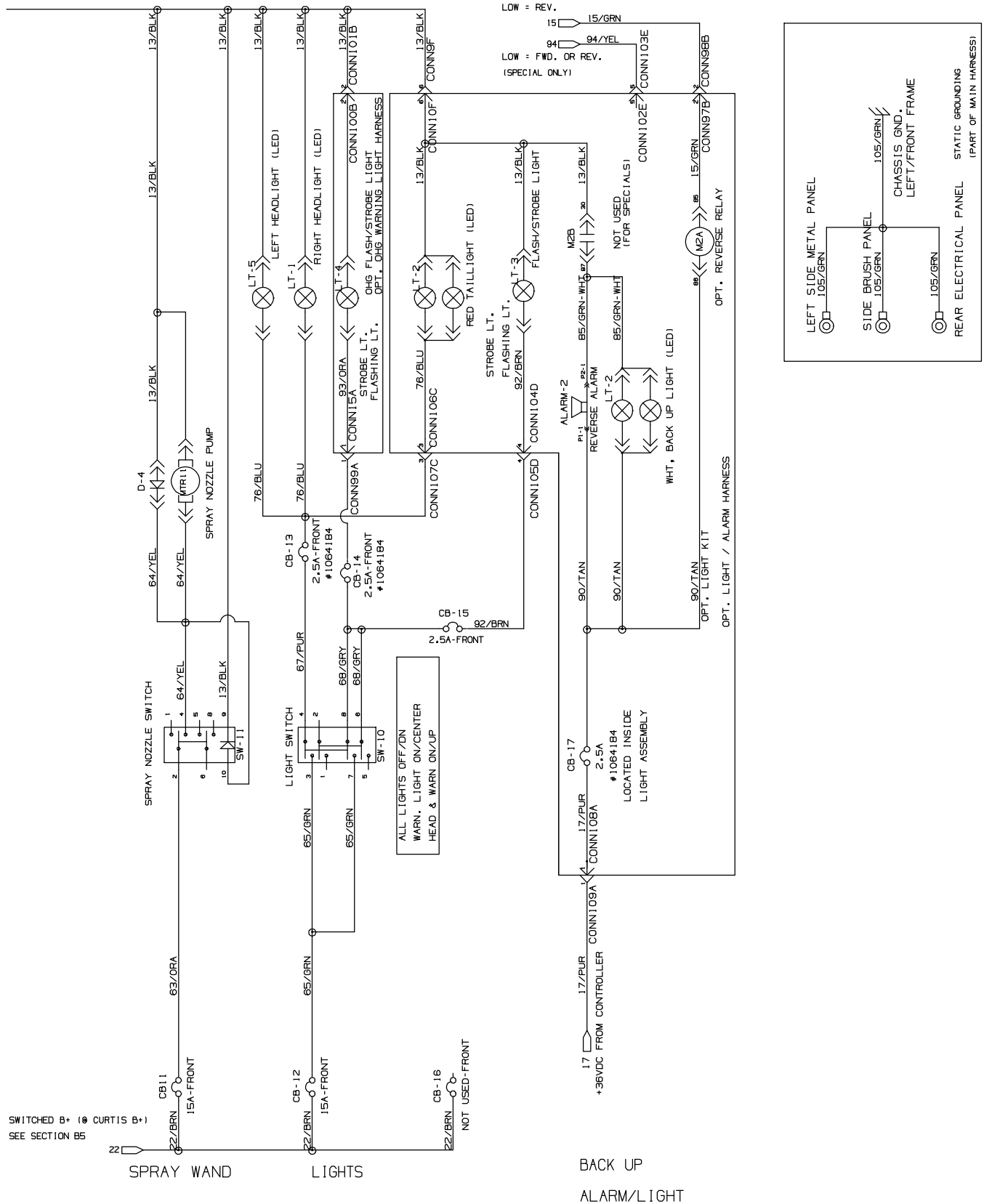
Fig. 25 – Electrical Schematic Group (S/N 30000000–30077834)
