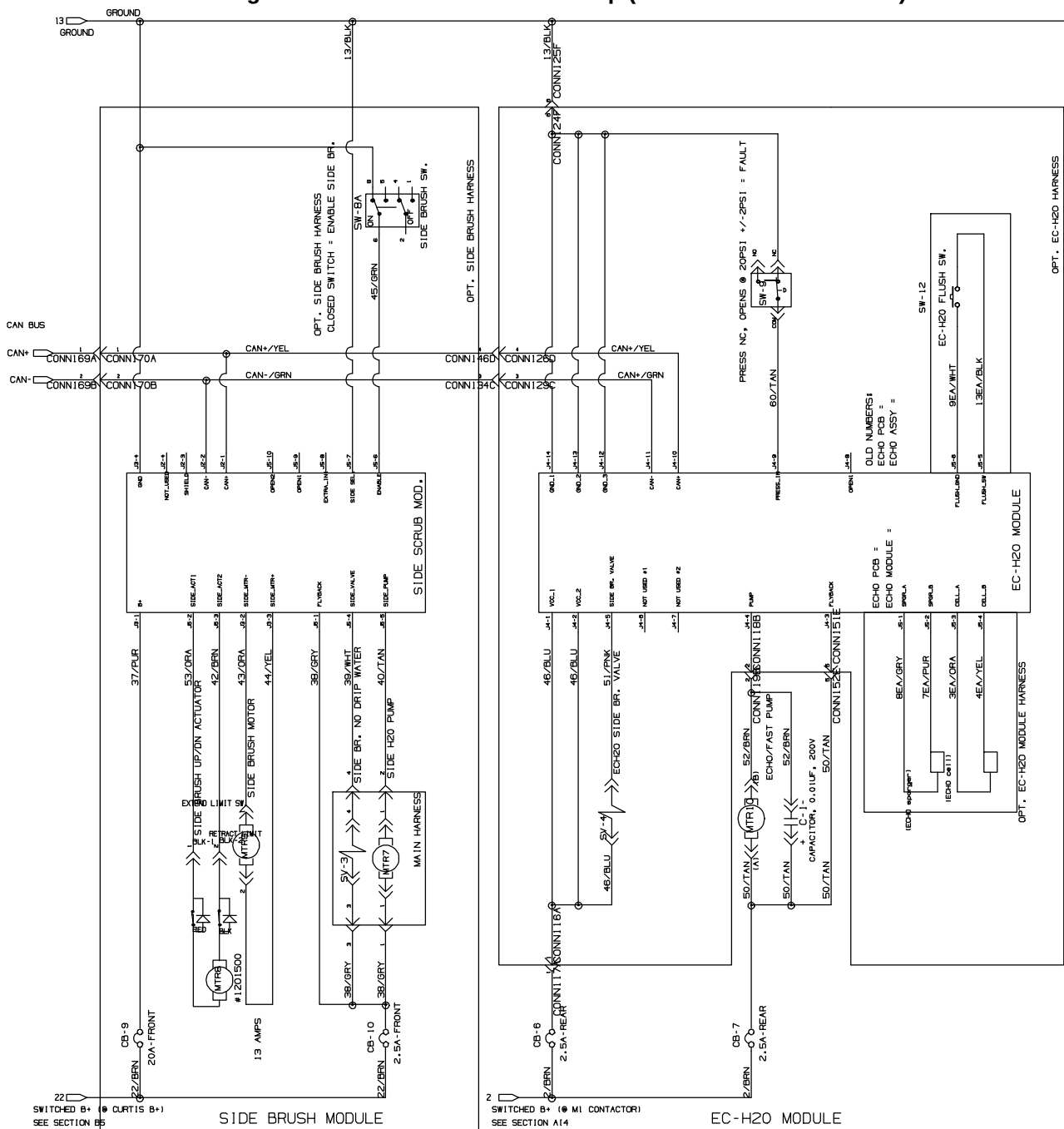
Fig. 26 – Electrical Schematic Group (S/N 30077835–39999999)
