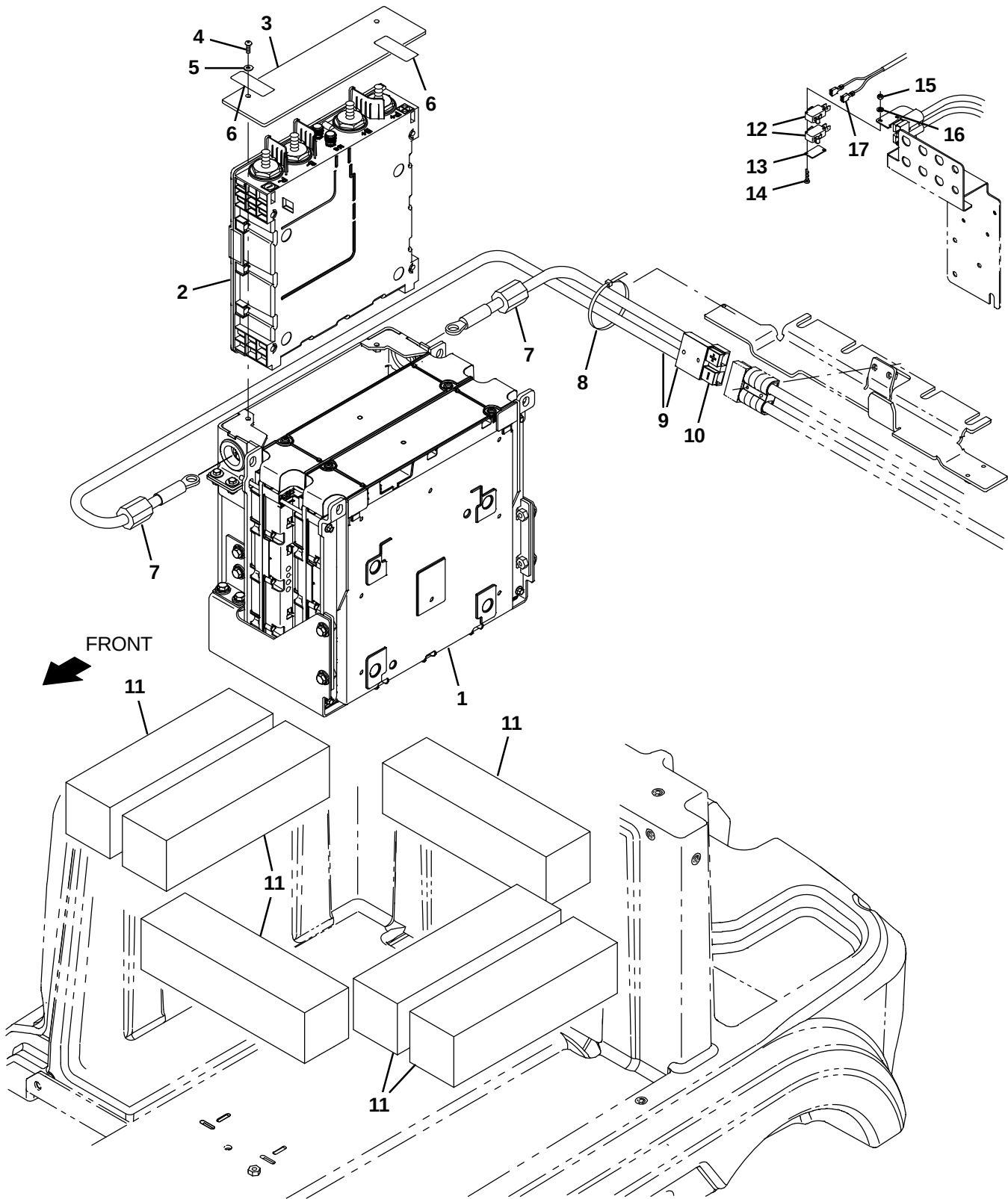
Fig. 26 – Battery Group, Lithium-Ion, 36V, 4.1 Kwh
