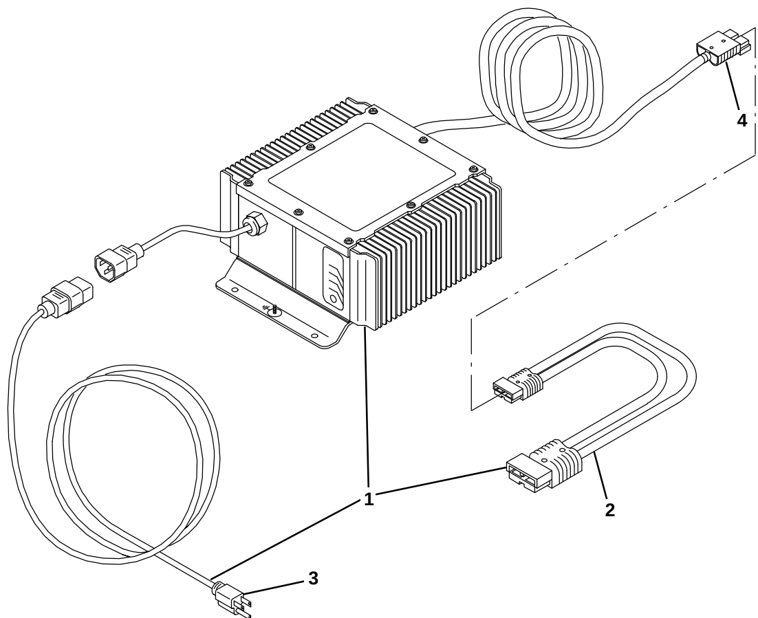
Fig. 29 – Battery Charger Group
