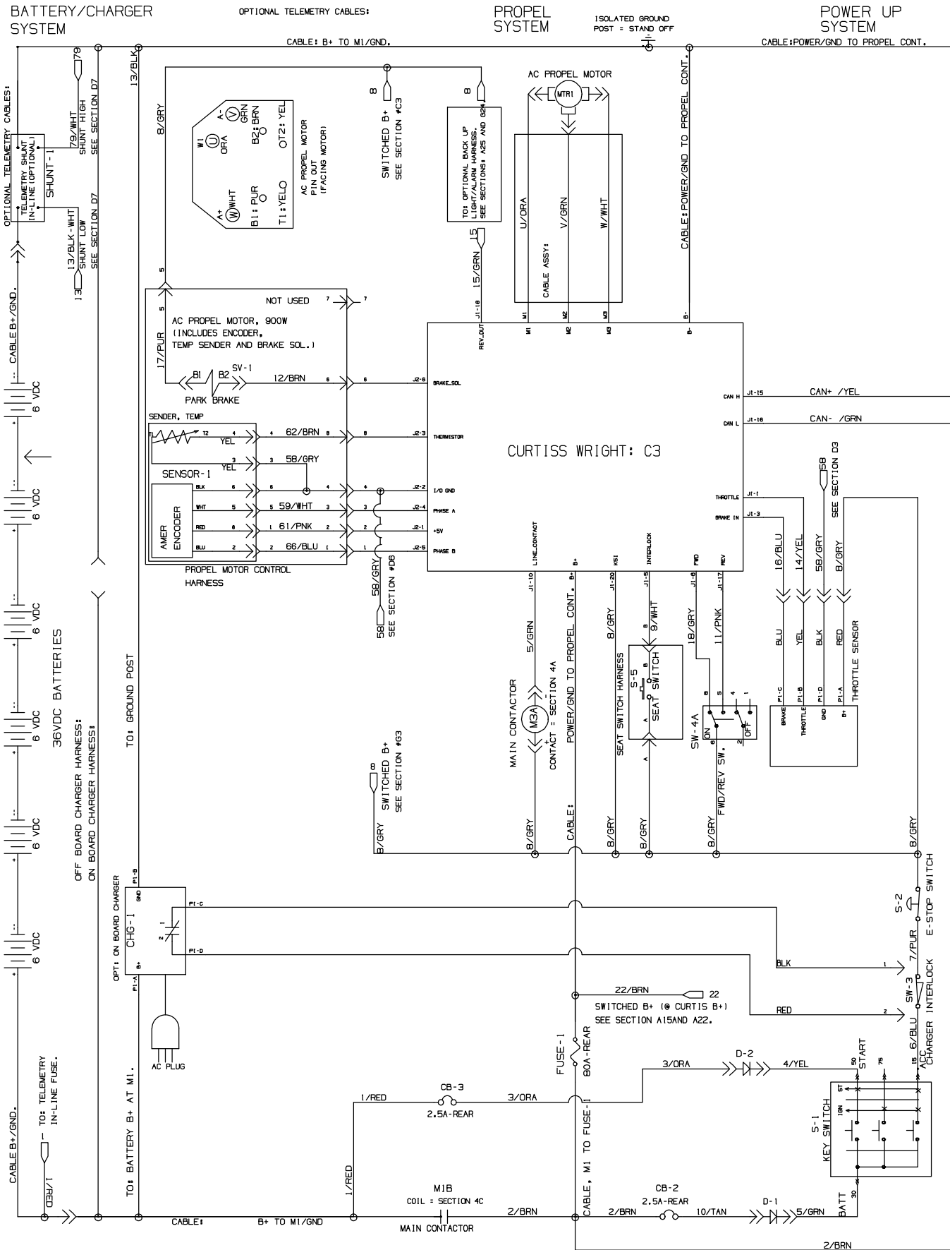
Fig. 26 – Electrical Schematic Group (S/N 10863998–19999999)
