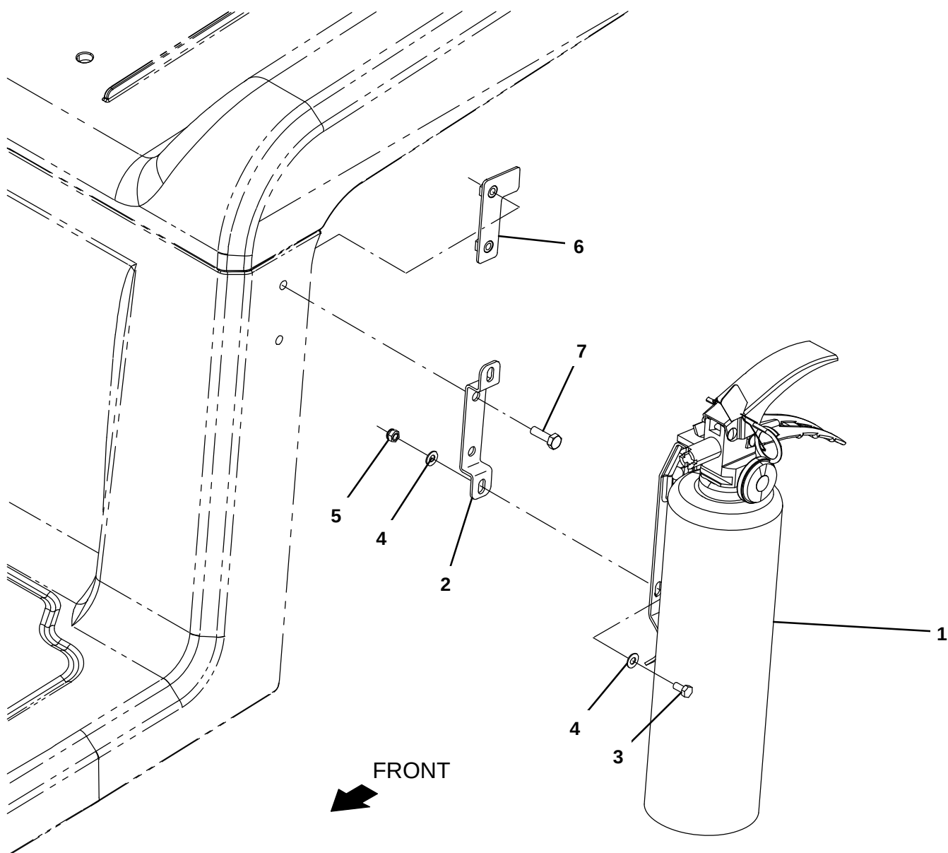
Fig. 40 – Fire Extinguisher Group
