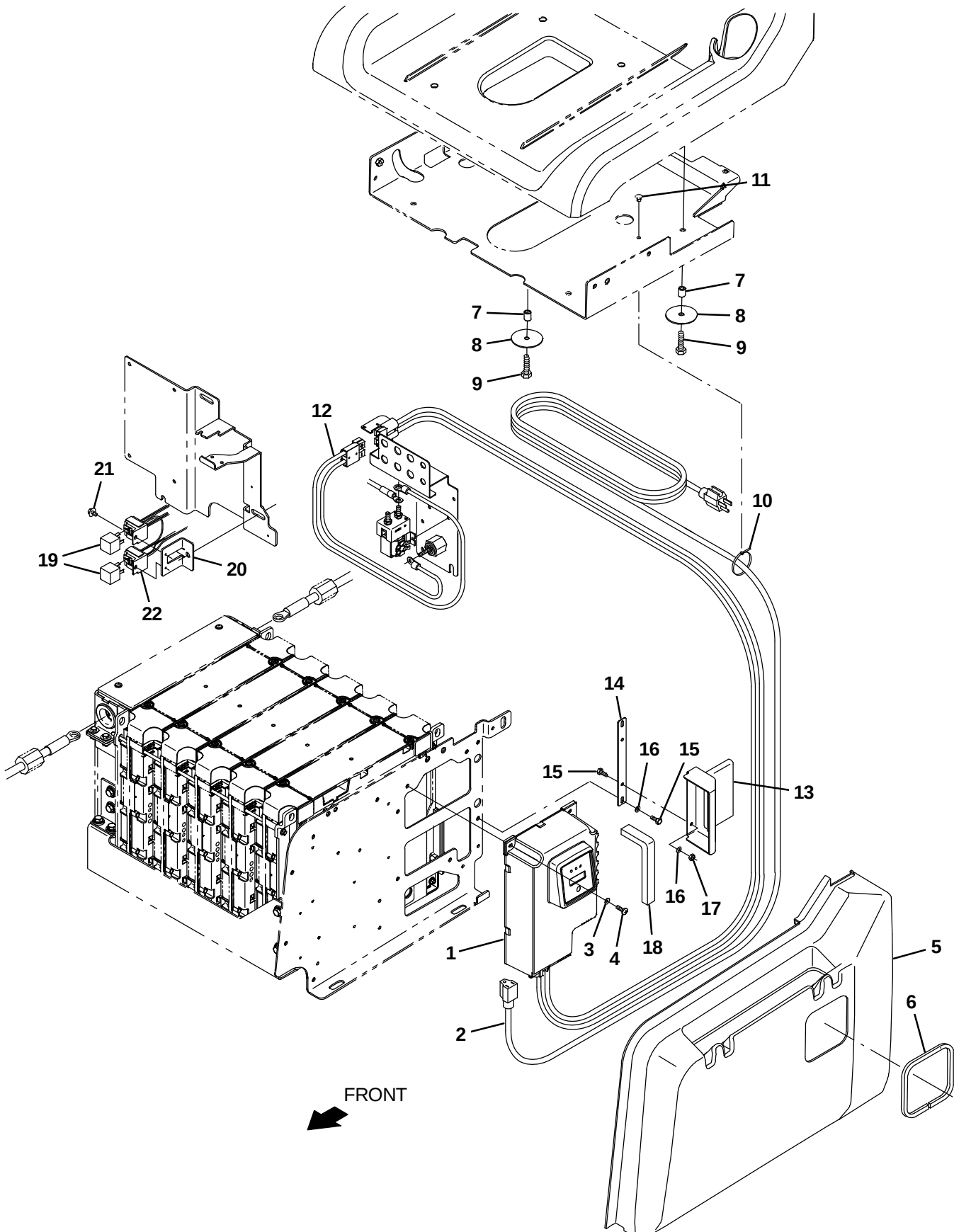
Fig. 35 – On-Board Battery Charger Group, Lithium-Ion
