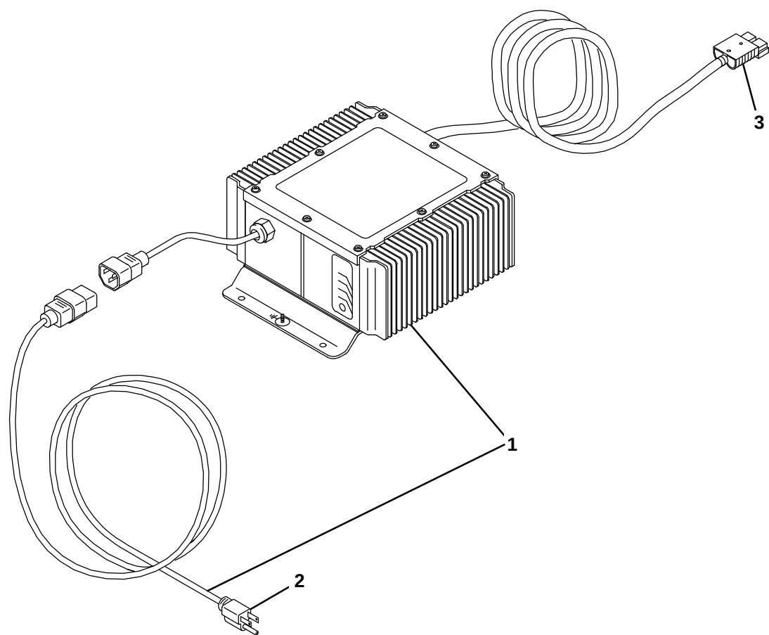
Fig. 28 – Battery Charger Group
