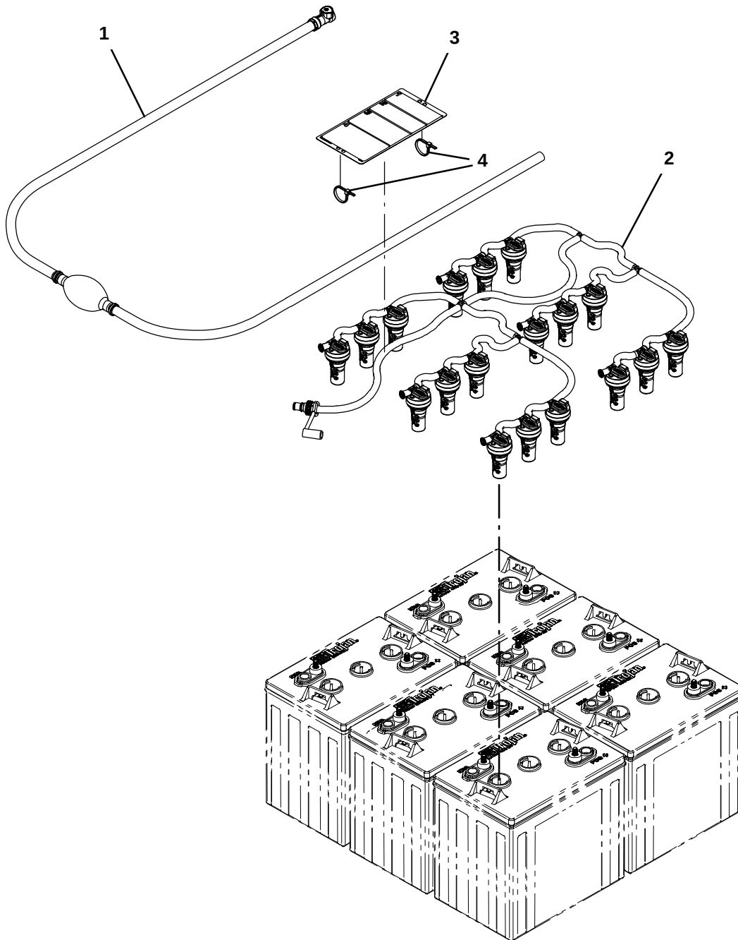
Fig. 38 – Manual Battery Watering System Kit
