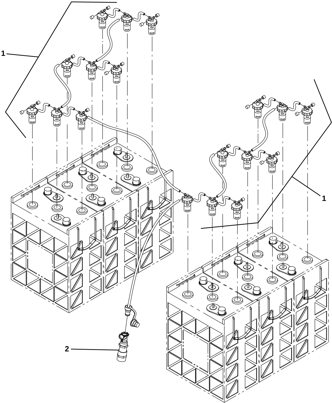
Fig. 36 – Flow-Rite™ Battery Water Manifold Kit
