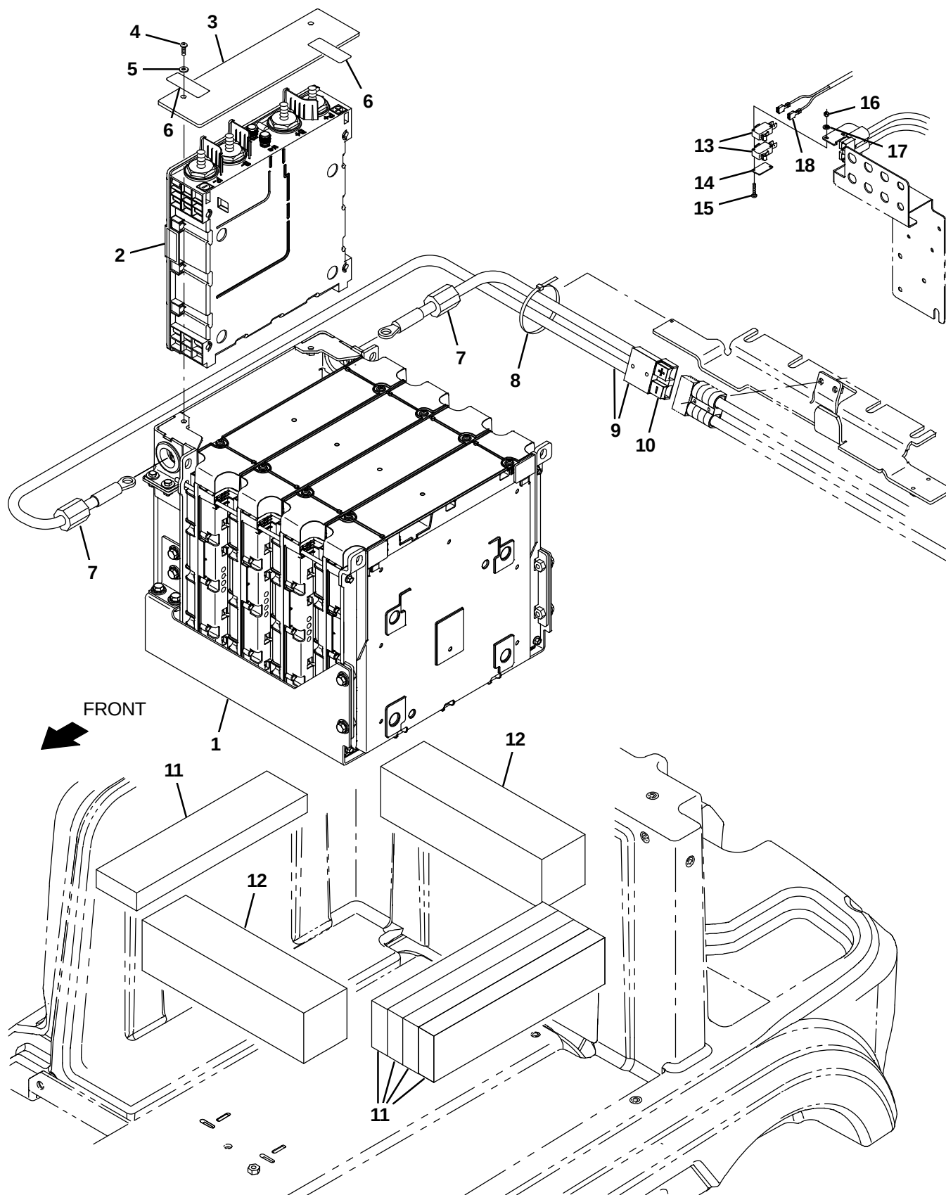
Fig. 25 – Battery Group, Lithium-Ion, 36V, 8.2 Kwh
