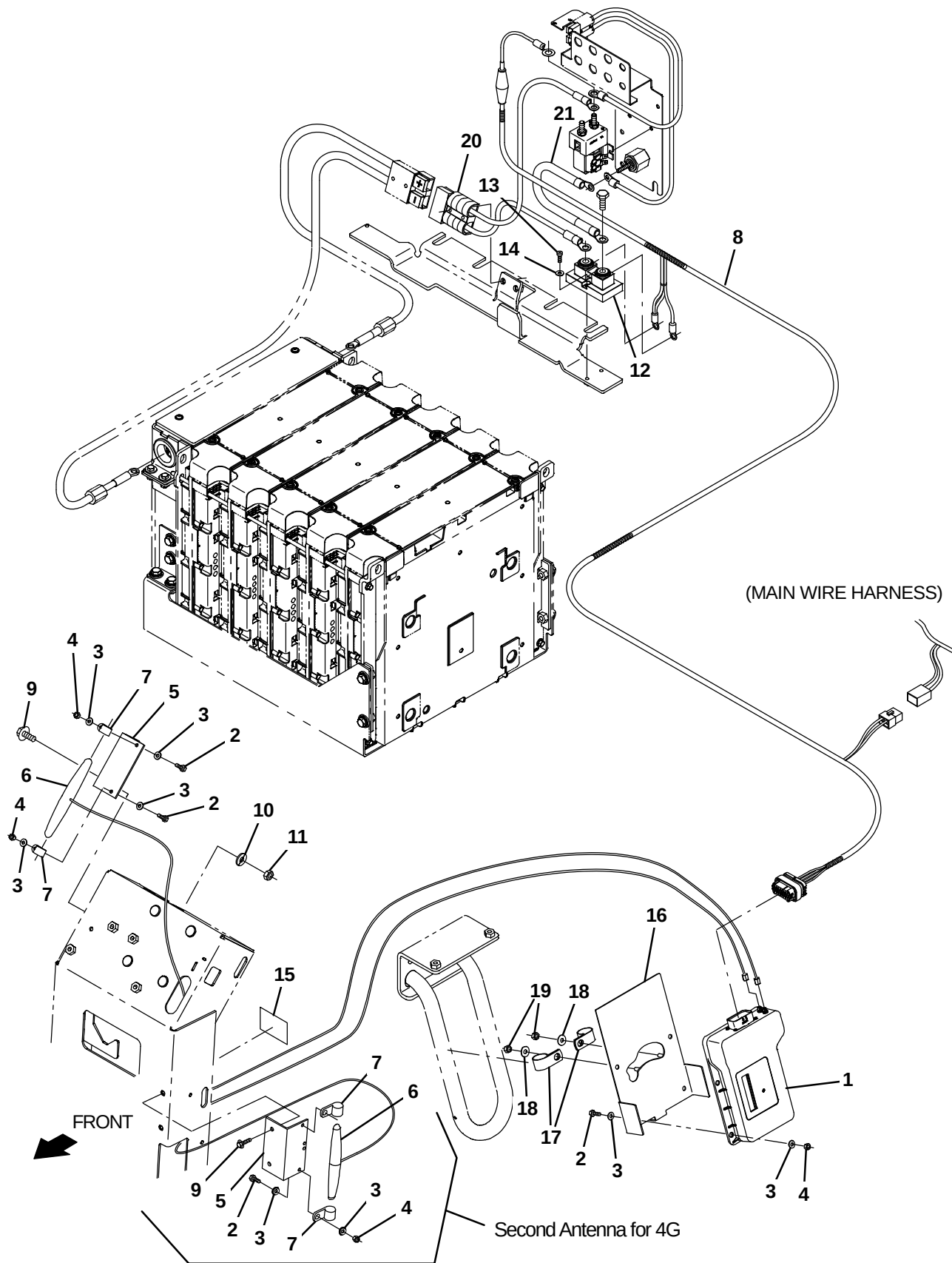
Fig. 21 – Telemetry Group, Lithium-Ion Battery (S/N 10967791–19999999)
