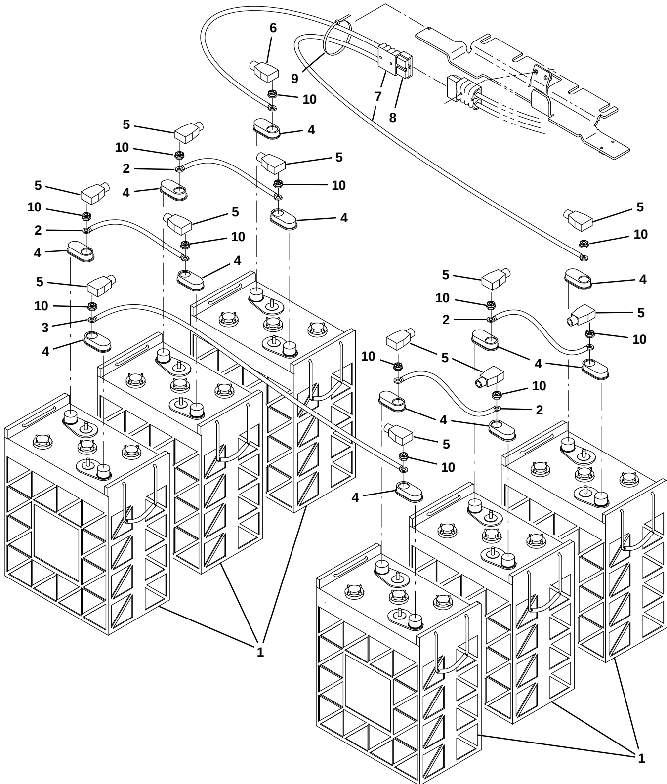
Fig. 22 – Battery Group, 36V 360Ah
