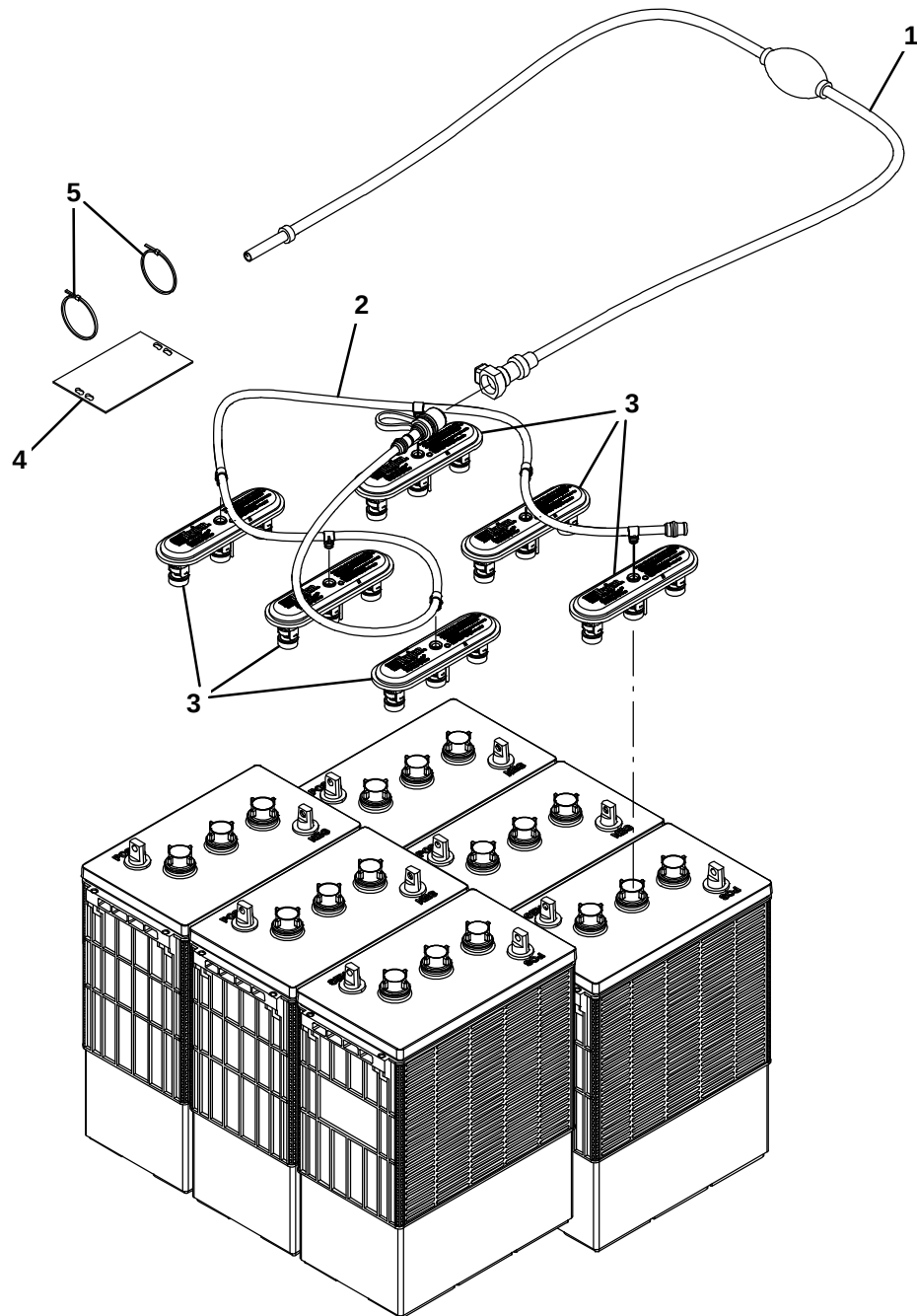
Fig. 37 – Hydrolink® Battery Watering System Kit
