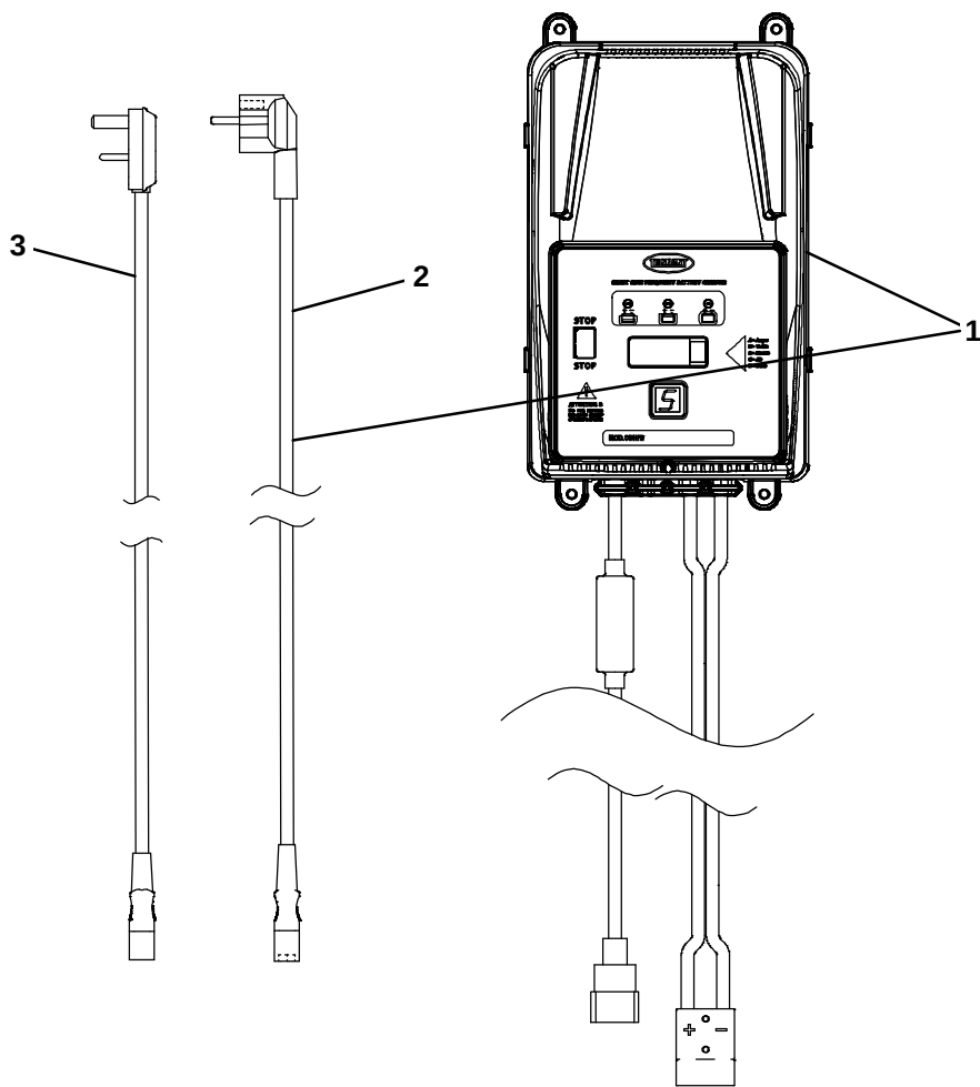
Fig. 31 – Battery Charger Group
