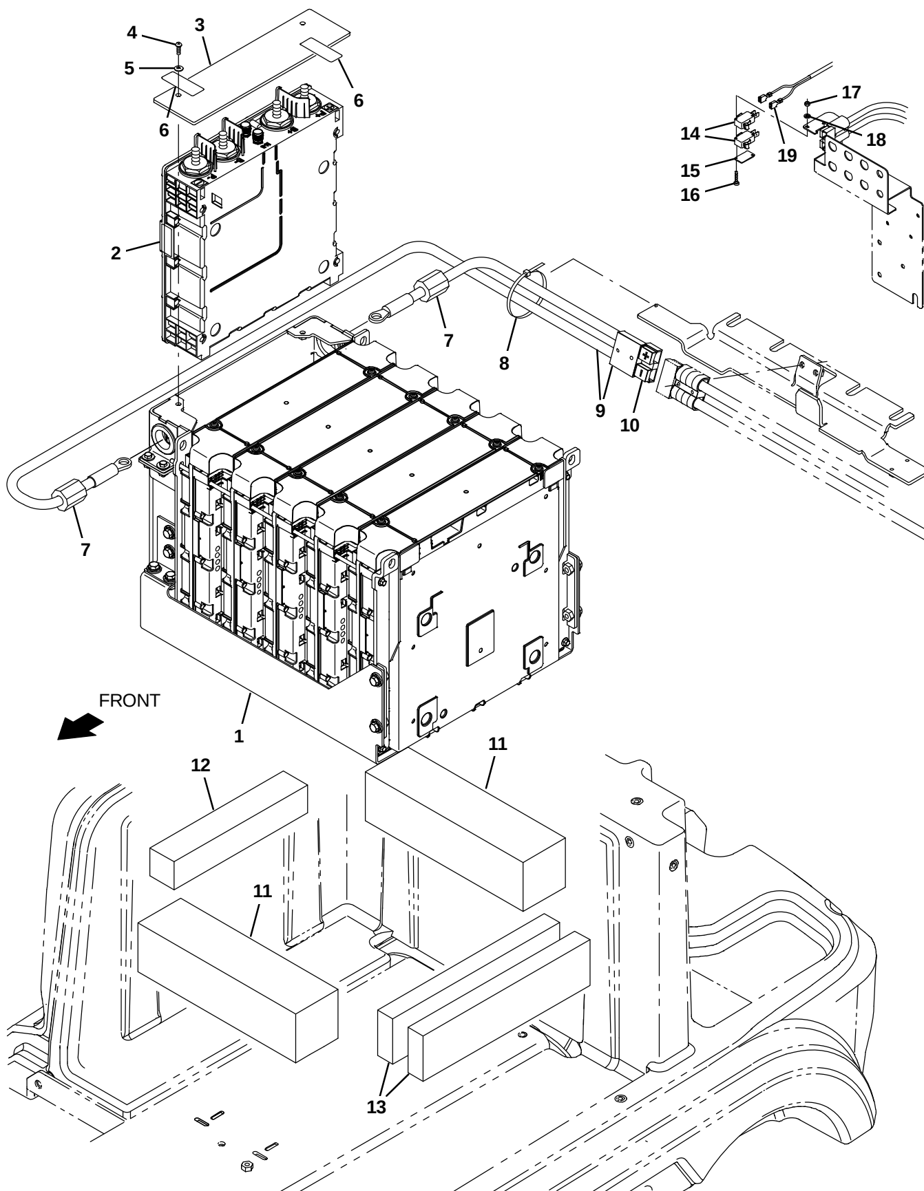
Fig. 24 – Battery Group, Lithium-Ion, 36V, 10.2 Kwh
