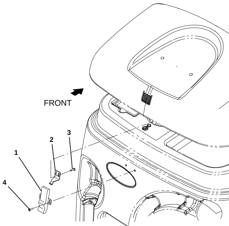
Fig. 39 – Transport Group
