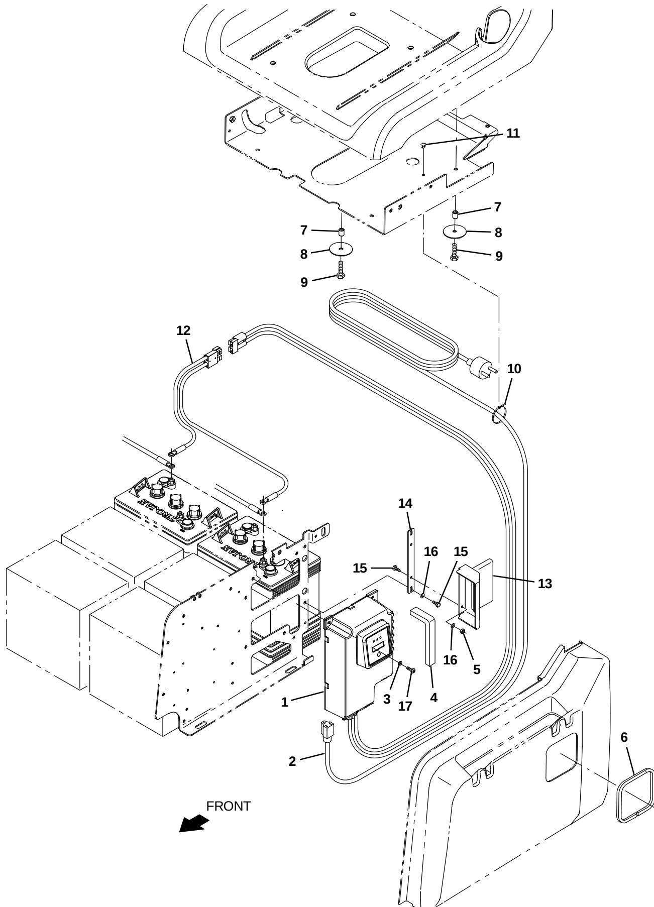
Fig. 34 – On-Board Charger Group, International
