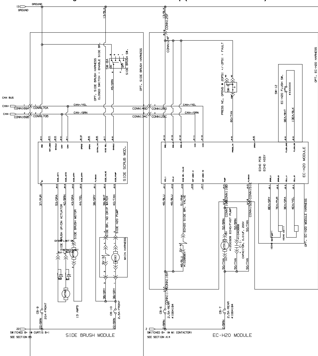
Fig. 25 – Electrical Schematic Group (S/N 10000000–10863997)
