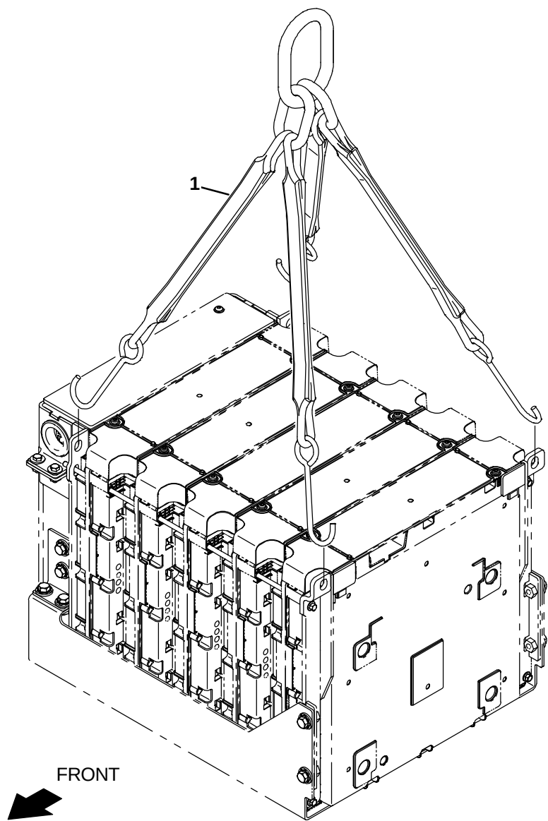
Fig. 27 – Lithium-Ion Battery Lifting Kit
