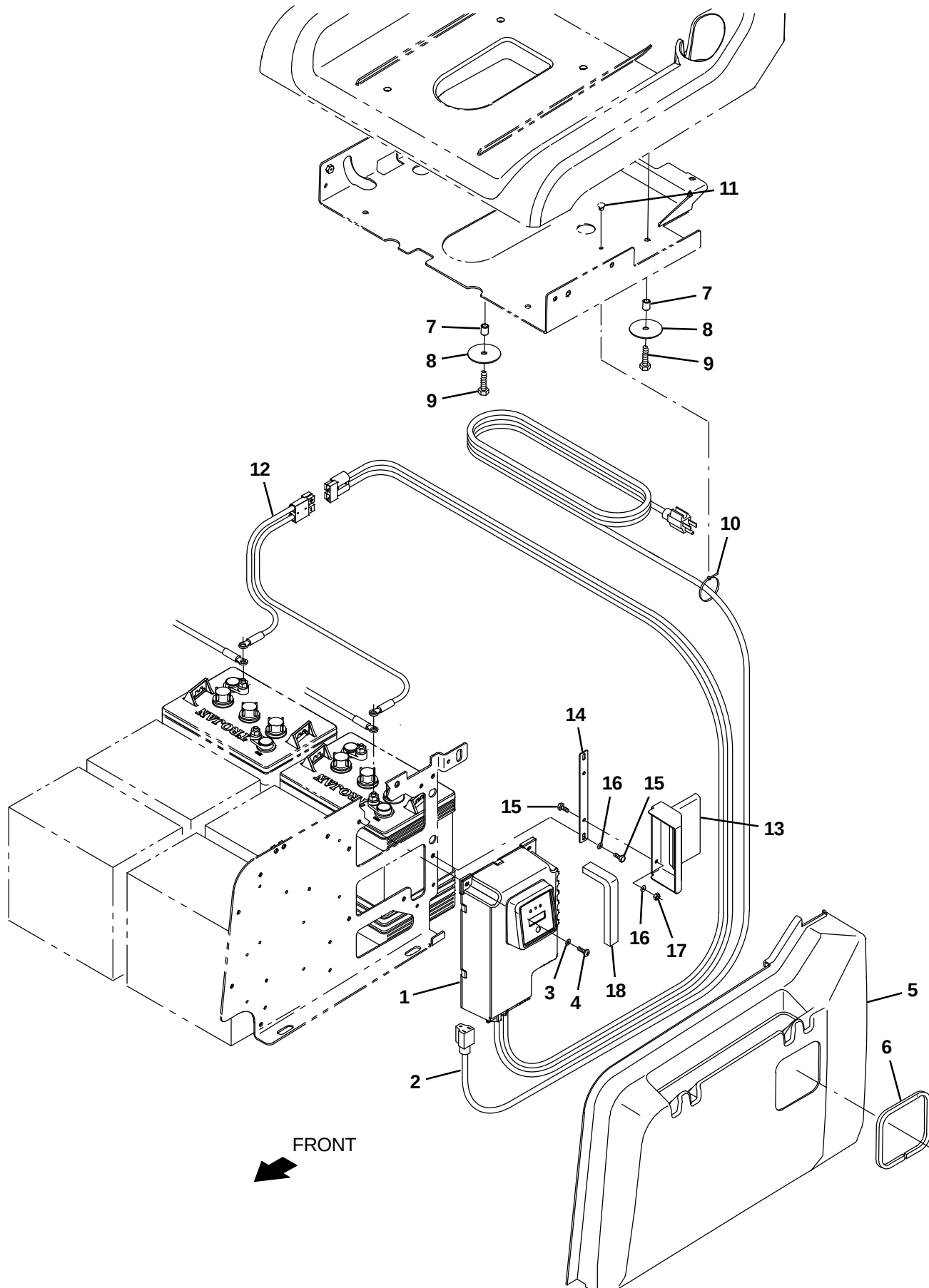
Fig. 33 – On-Board Charger Kit
