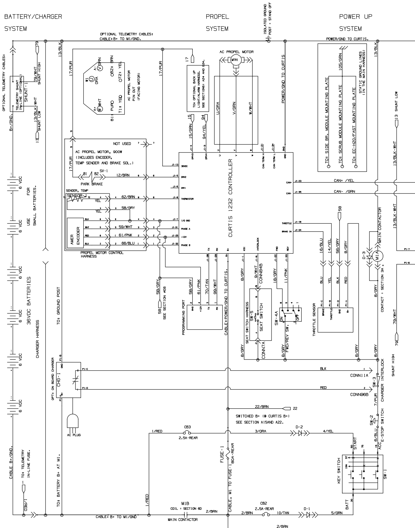
Fig. 25 – Electrical Schematic Group (S/N 10000000–10863997)
