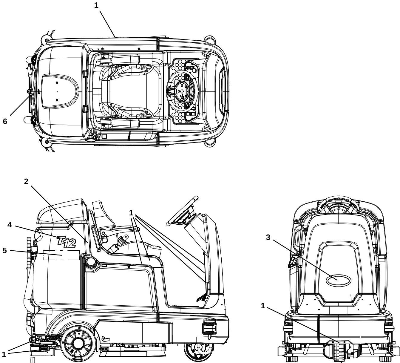
Fig. 28 – Labels Group
