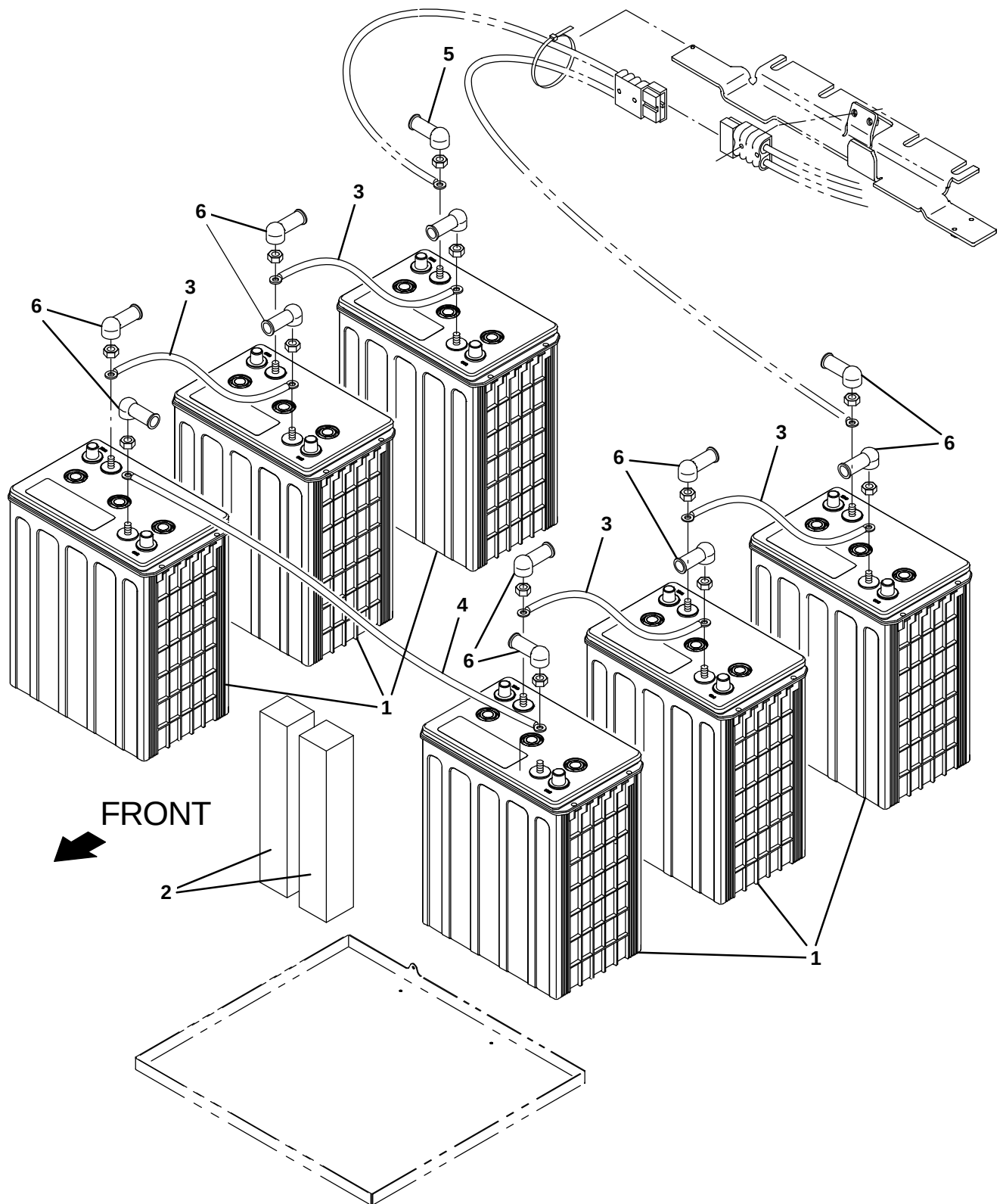
Fig. 23 – Battery Group, 36V 312Ah
