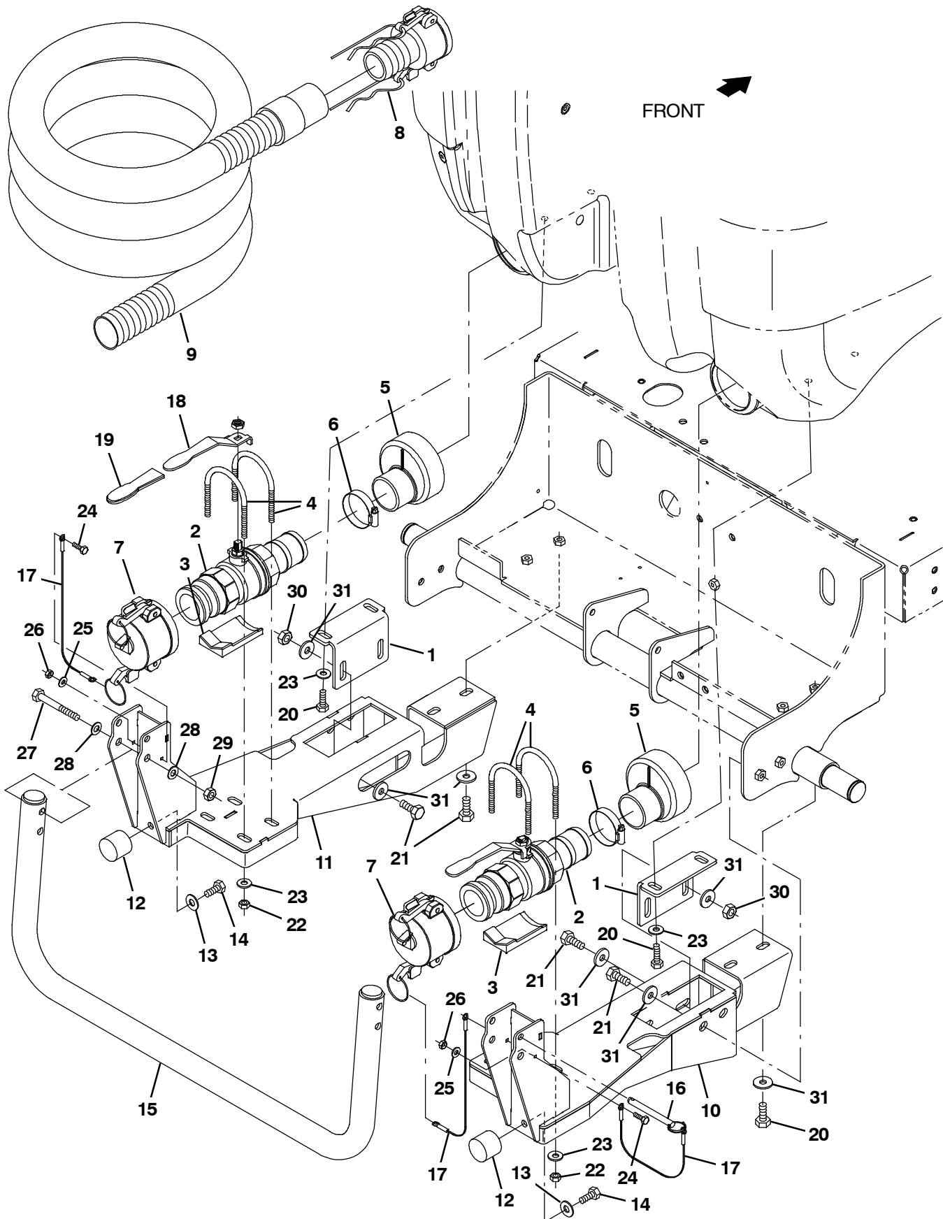
Fig. 58 - Positive Drain Valve Group
