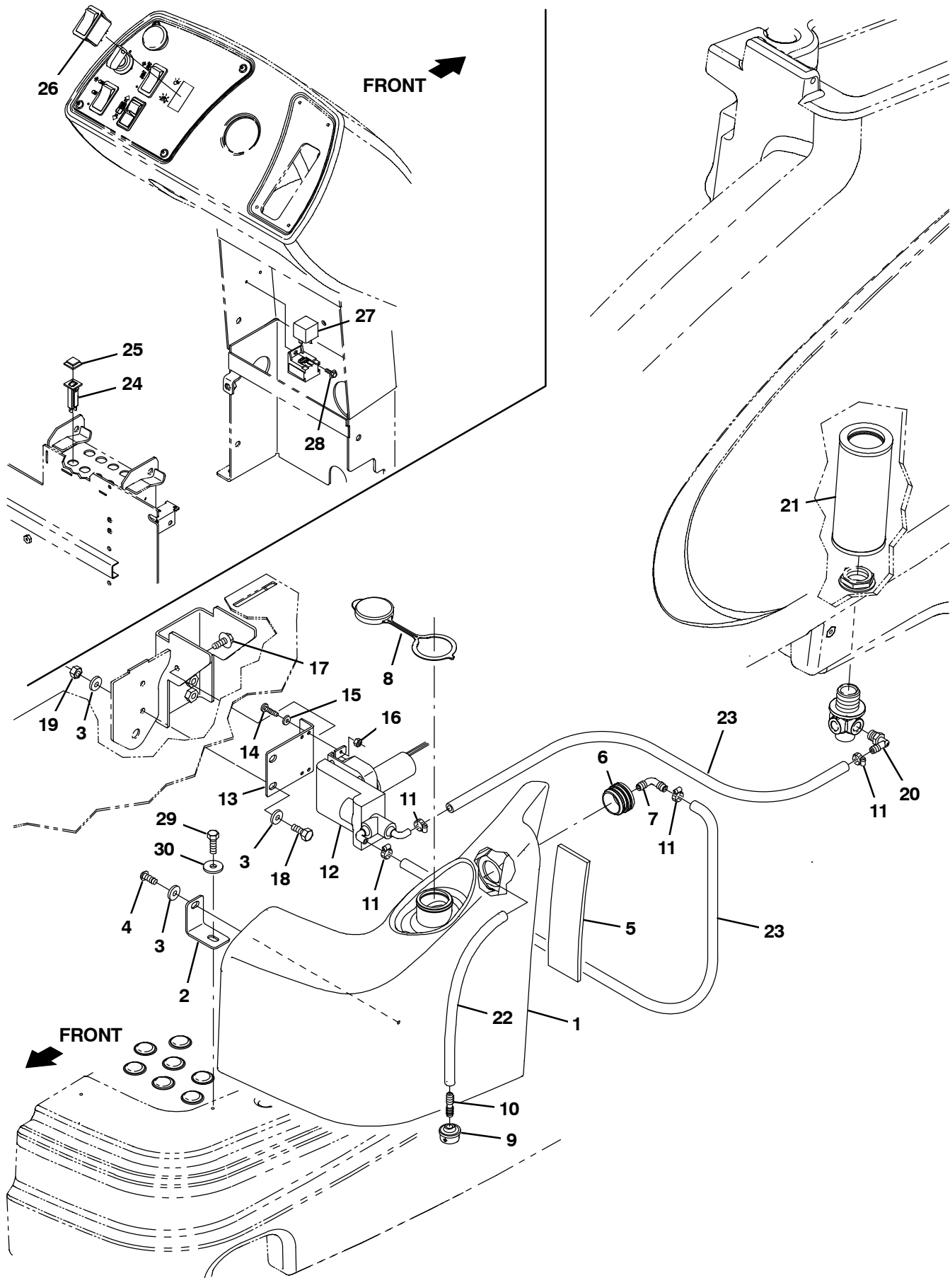
Fig. 57 – Severe Environment/Detergent Metering Group
