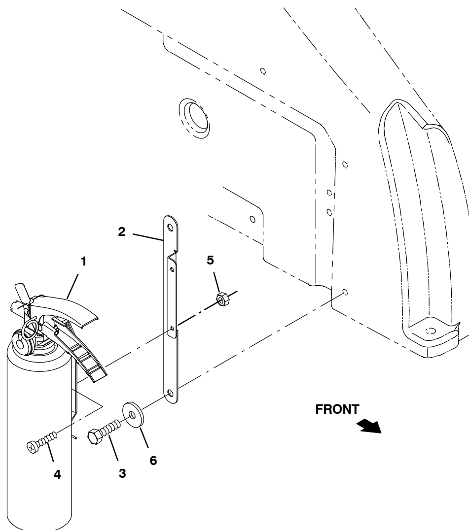
Fig. 55 – Fire Extinguisher Kit
