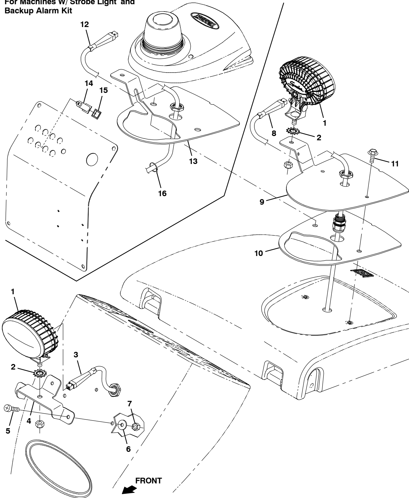
Fig. 59 – Spotlight Kit, Blue
