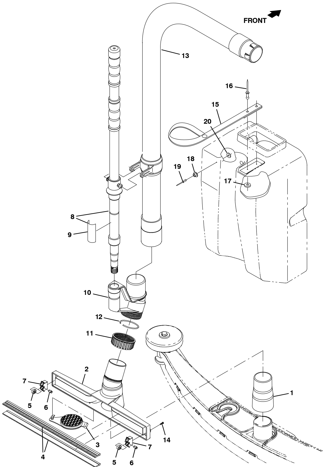
Fig. 19 – Vacuum Wand Kit
