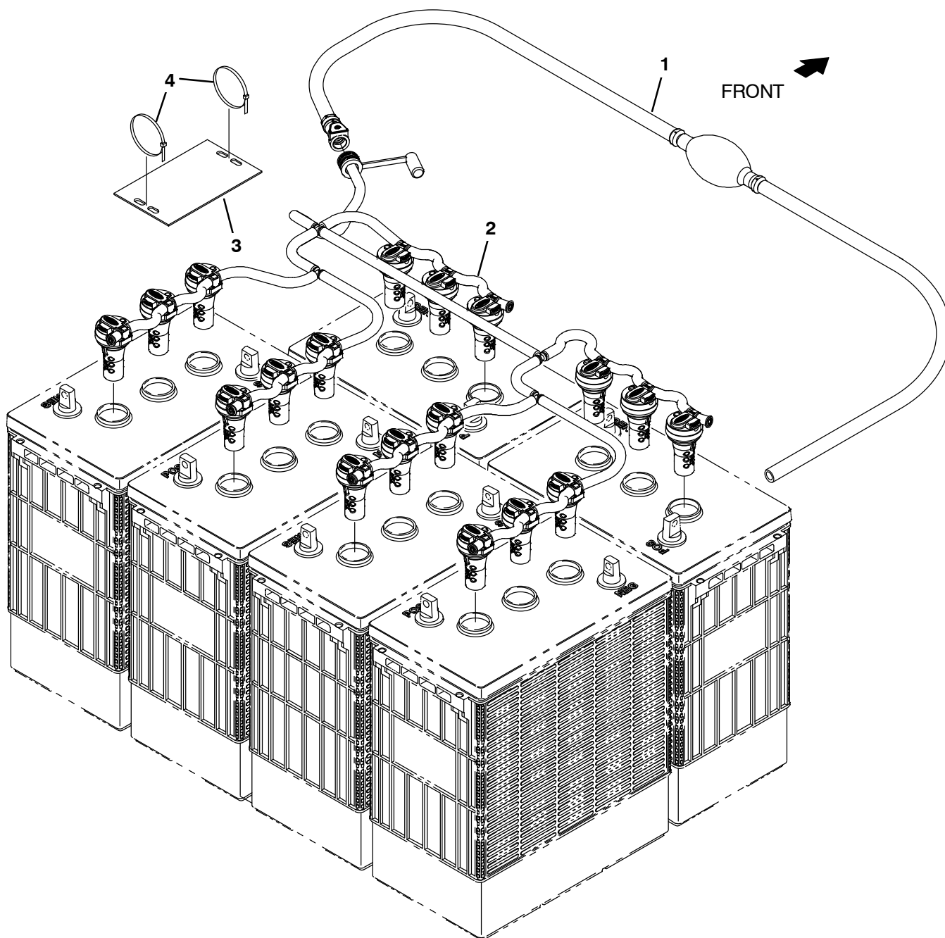
Fig. 54 – Manual Battery Watering System
